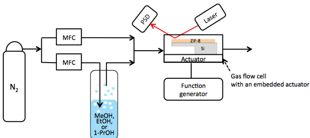
Figure S1. Schematic illustration of the instrument set-up.
