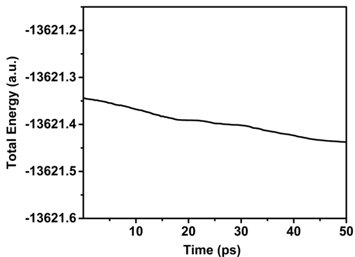
Figure S1 Time-evolution of the total energy of the Au 18 /TiO 2 system during the soft-landing process of Au 18 onto TiO 2 (110) surface.
