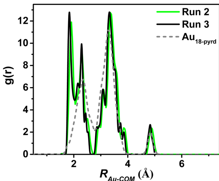
Figure S3 Computed g(r) functions of the Au-COM distance for the pre-collision period ( t < 1 ps) from the second and the third BOMD simulation Run 2 (green line) and Run 3 (black line). The dashed gray line shows the g(r) functions for the bare \text{Au}_{18} -pyrd cluster (without \text{TiO}_2 support).
