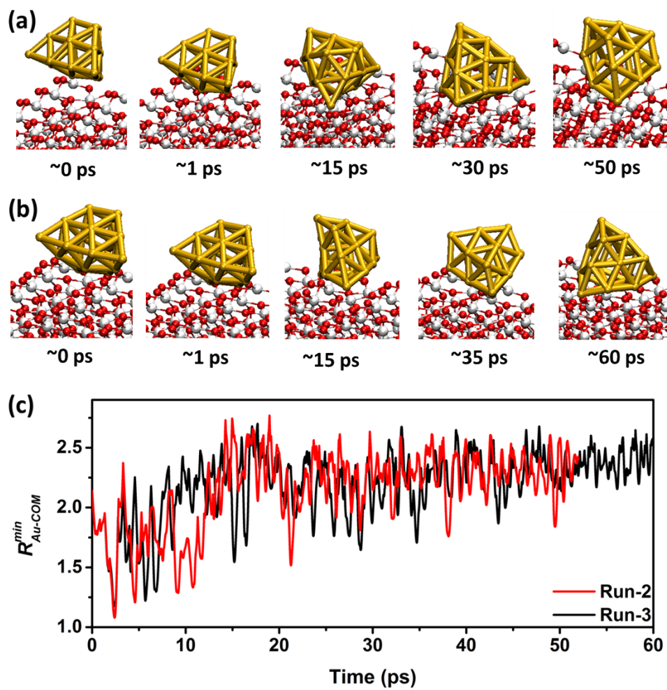
Figure S2 (a) and (b) present the snapshot structures from two independent BOMD simulations (Run-2 and Run-3, respectively) of the soft-landing of the Au 18 cluster onto the TiO 2 (110) surface. (c) Time-evolution of minimum distance of the Au atoms relative to the center of the mass (COM) of the Au 18 ( R_{Au-COM}^{min} ).
