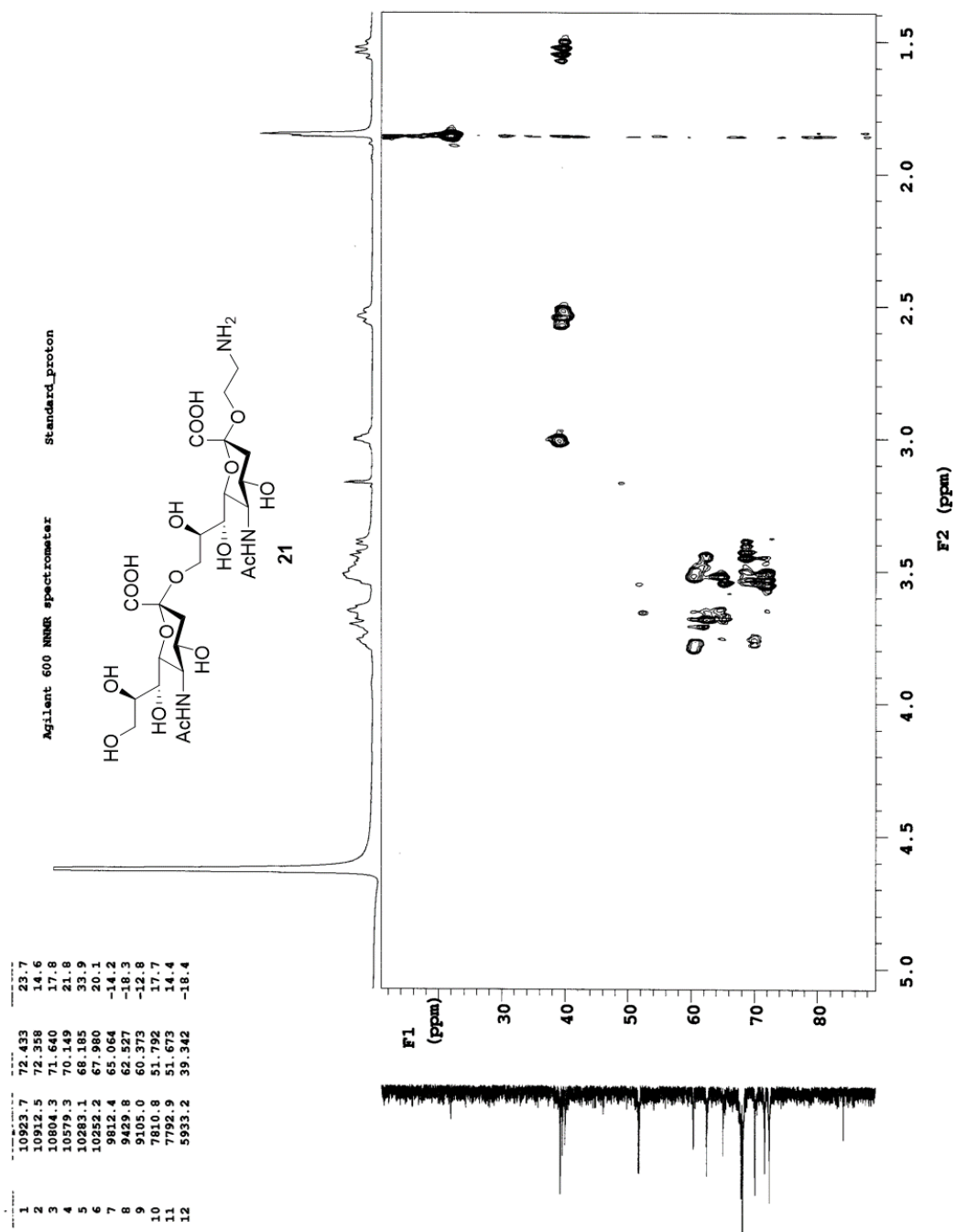
1 H- 13 C HMQC Spectrum of compound 15 (D 2 O, 600 MHz)
