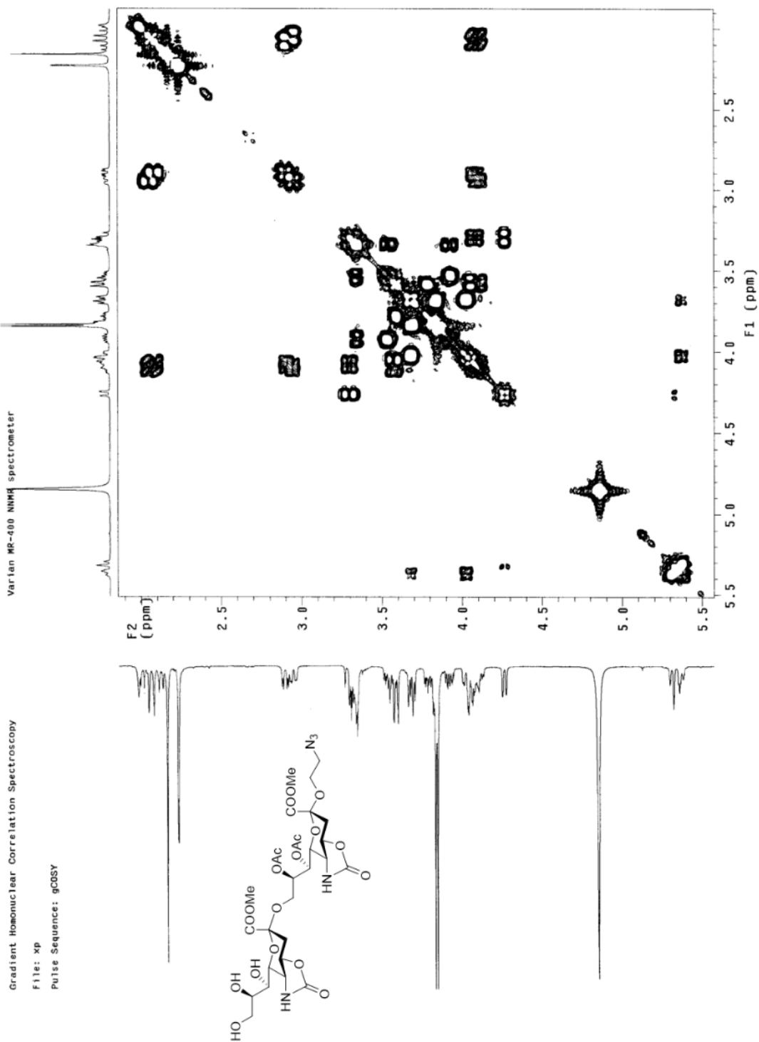
^1\text{H} - ^1\text{H} COSY Spectrum of compound 14 (CD 3 OD, 400 MHz)
