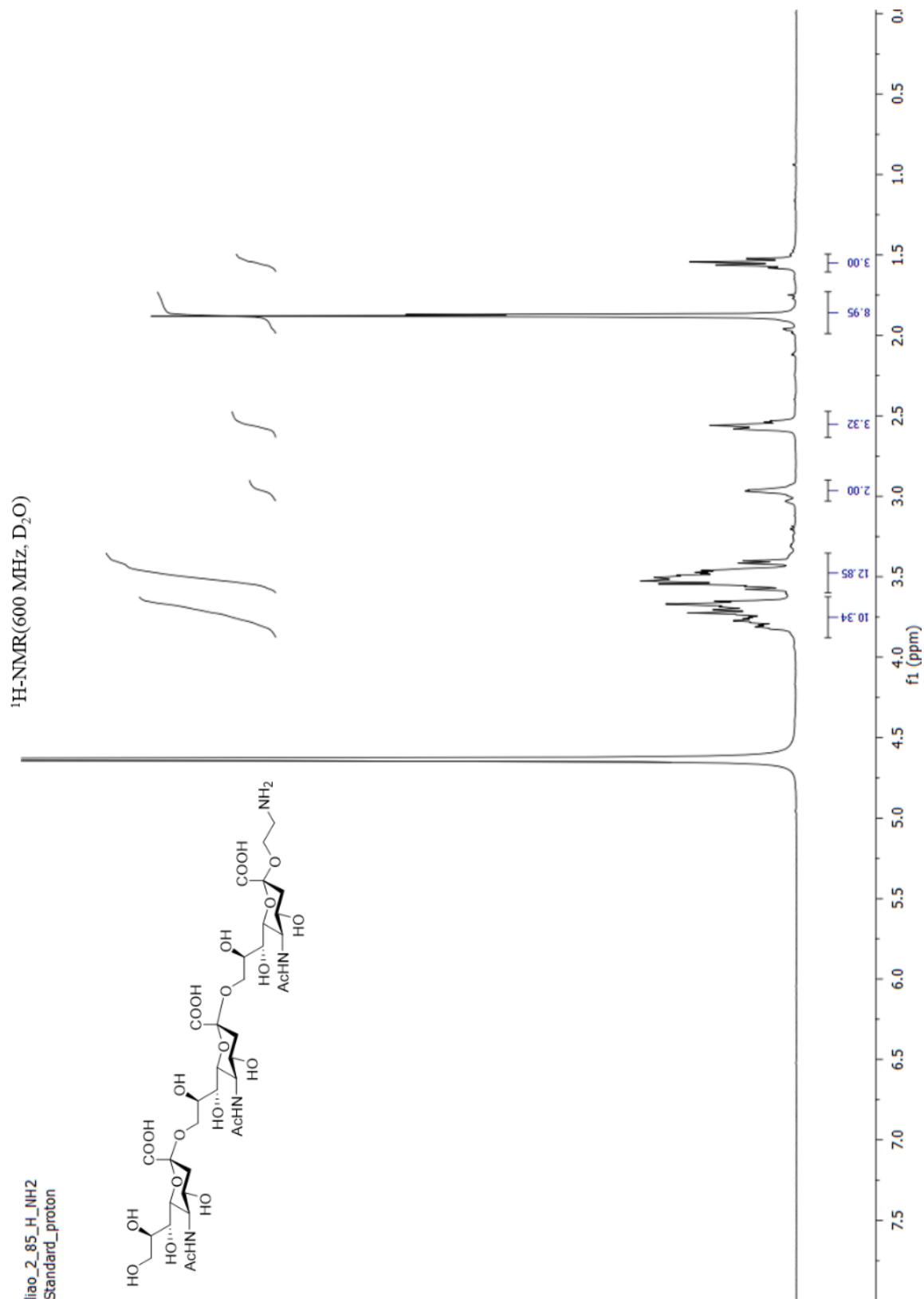
1 H NMR Spectrum of compound 17 (D 2 O, 600 MHz)
