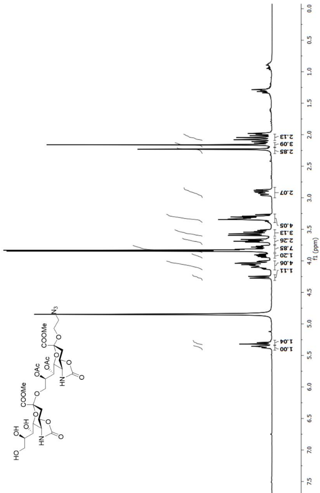
^1\text{H} NMR Spectrum of compound 14 ( \text{CD}_3\text{OD} , 400 MHz)
