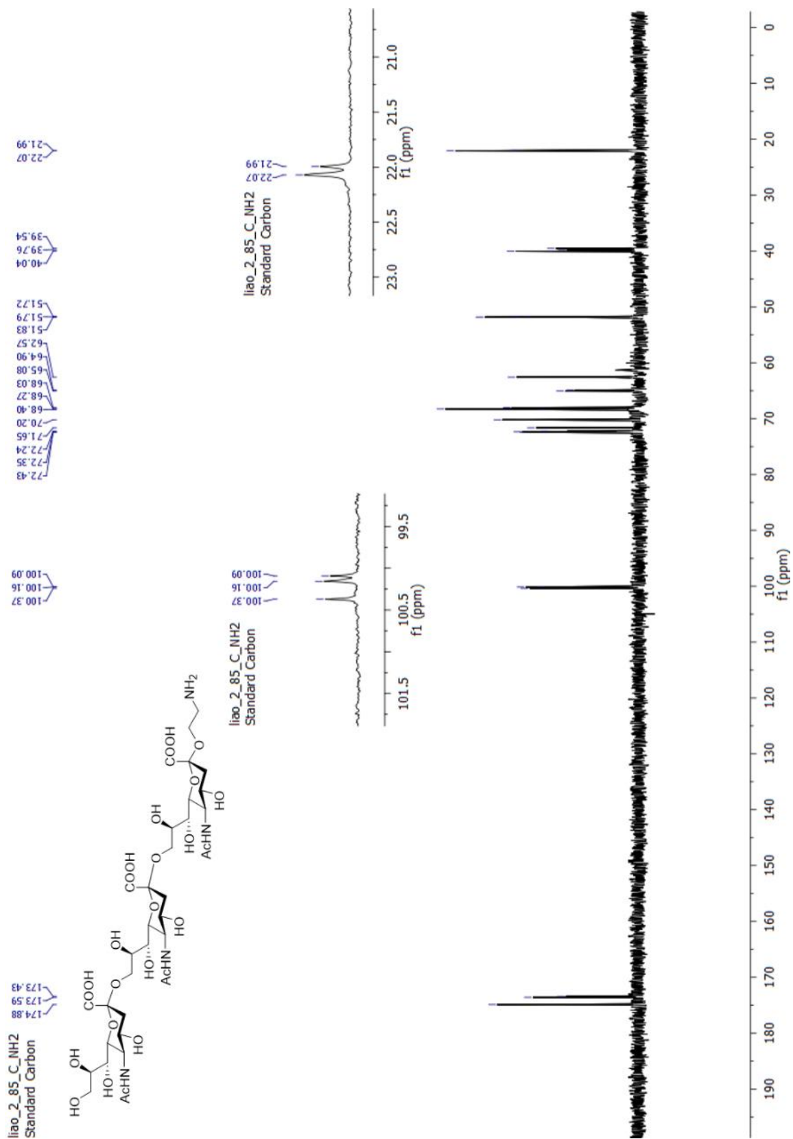
13 C NMR Spectrum of compound 17 (D 2 O, 150 MHz)
