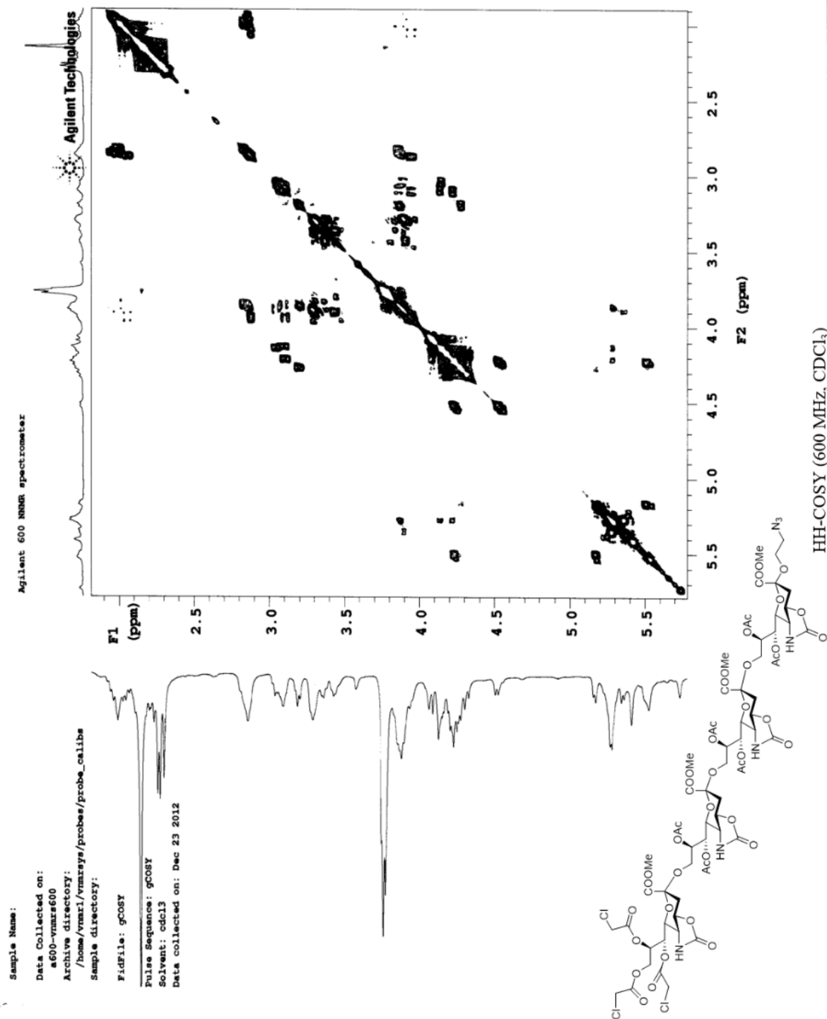
^1\text{H} - ^1\text{H} COSY Spectrum of compound 18 (CDCl 3 , 600 MHz)
