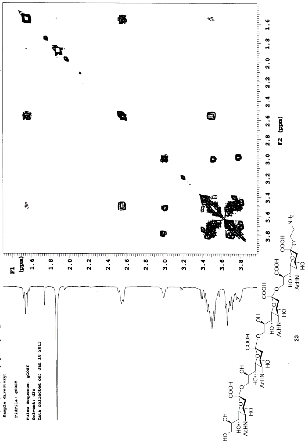
^1\text{H} - ^1\text{H} COSY Spectrum of compound 19 ( \text{D}_2\text{O} , 600 MHz)
