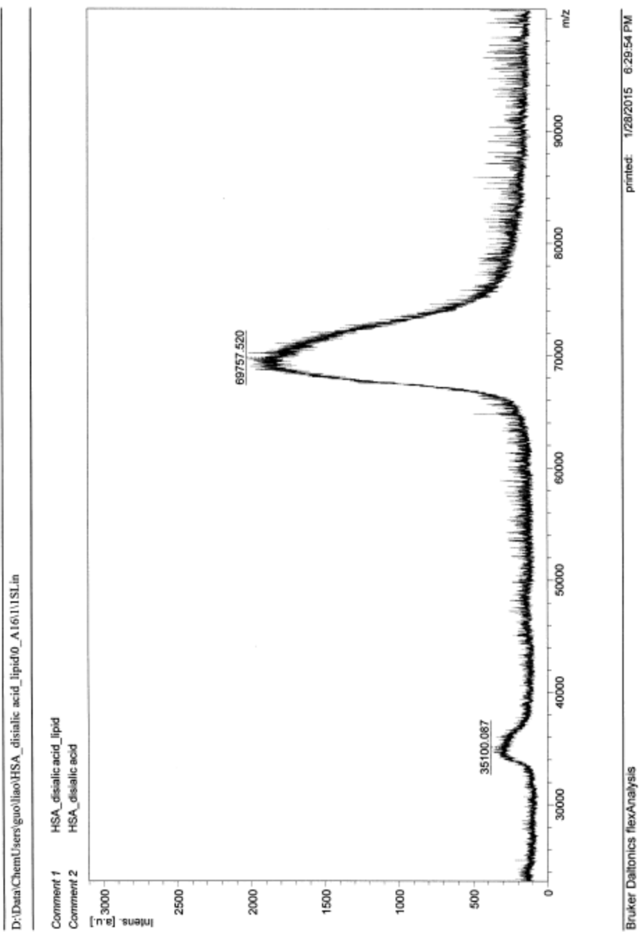
MALDI TOF MS spectrum of conjugate 5
