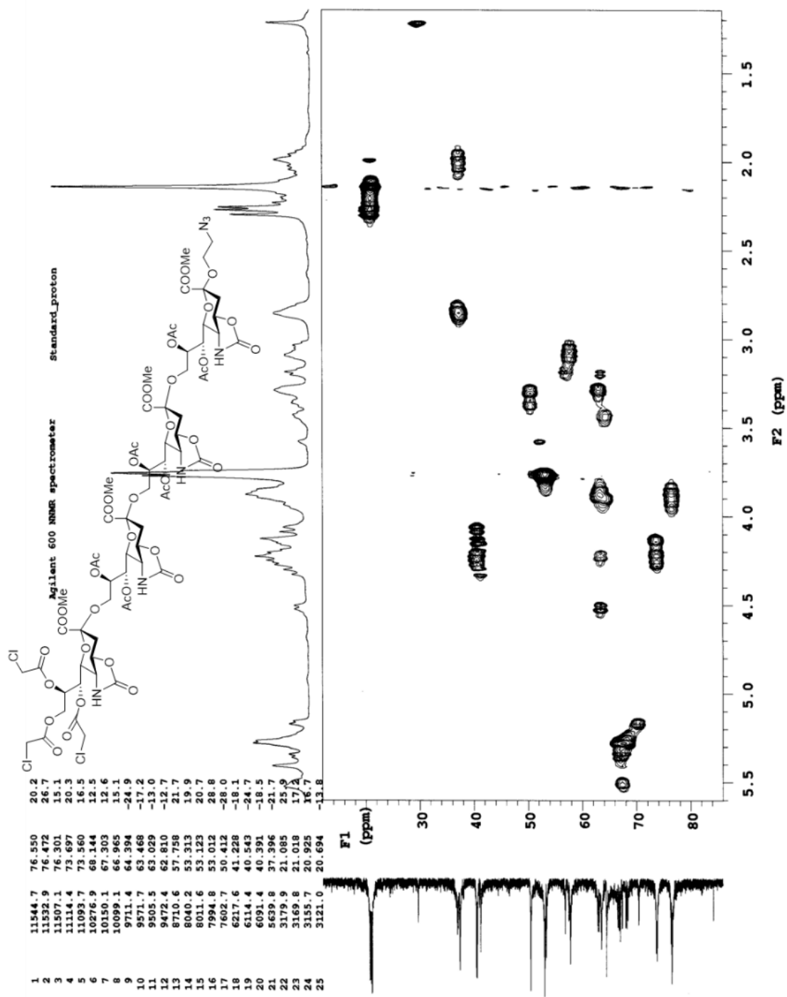
^1\text{H} - ^{13}\text{C} HMQC Spectrum of compound 18 ( \text{CDCl}_3 , 600 MHz)
