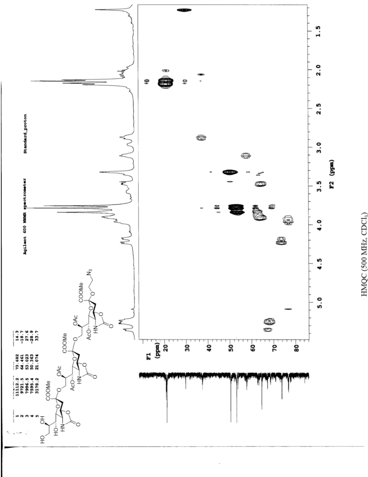
^1\text{H} - ^{13}\text{C} HMQC Spectrum of compound 16 ( \text{CDCl}_3 , 500 MHz)
