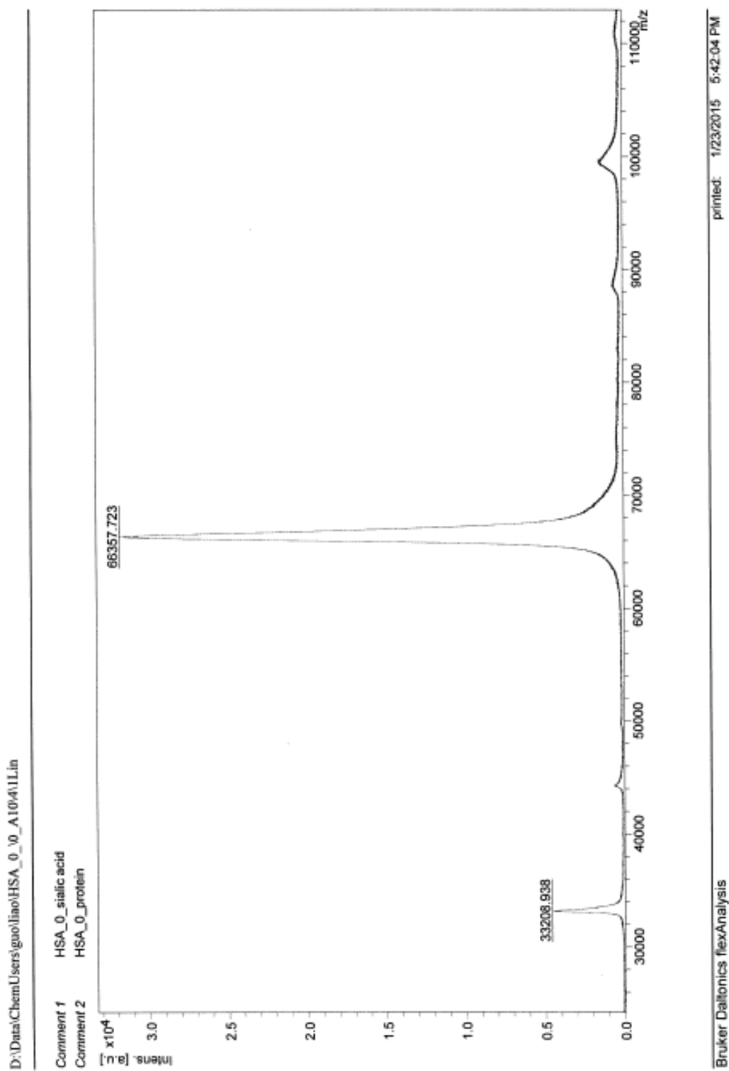
MALDI TOF MS spectrum of HSA protein
