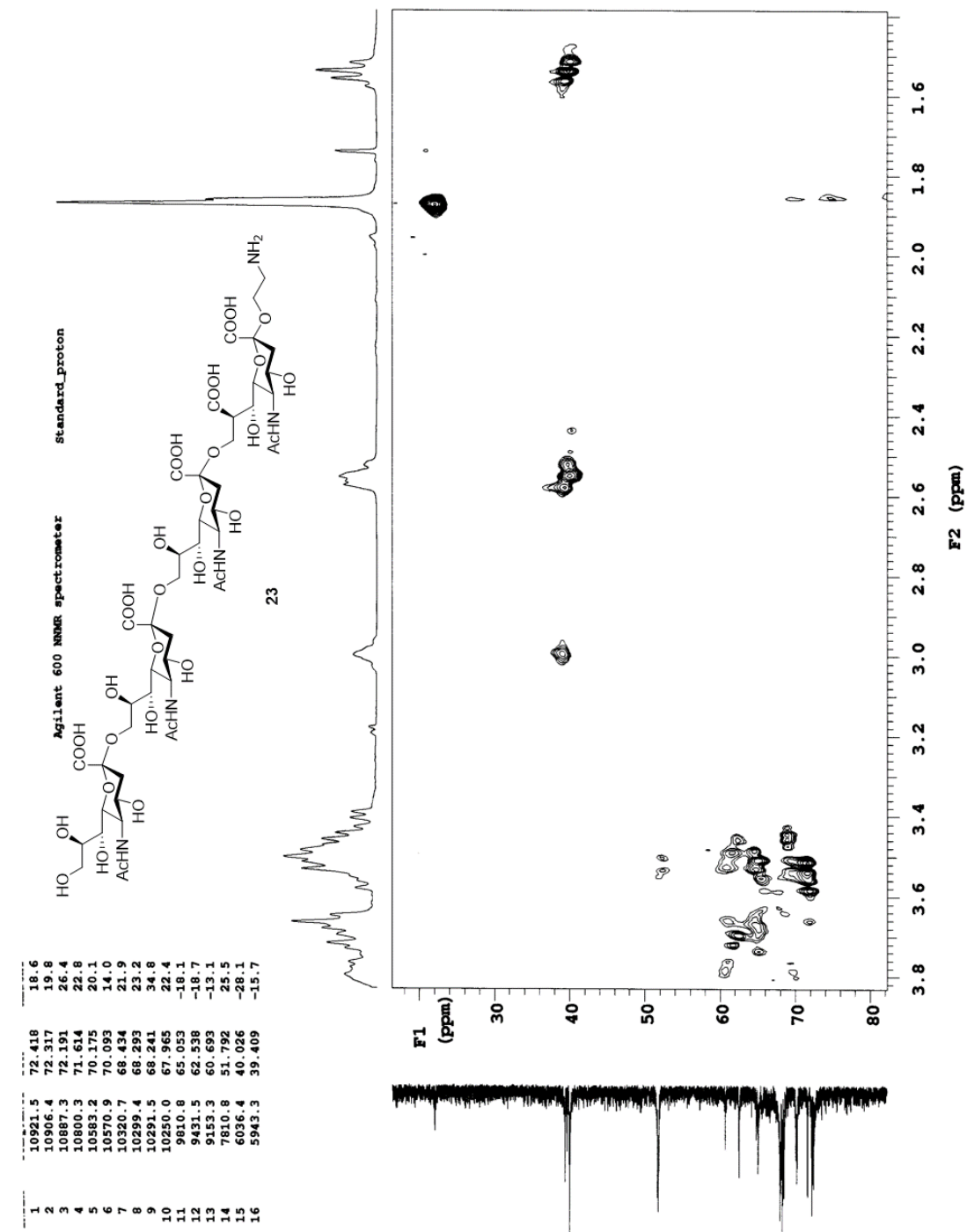
1 H- 13 C HMQC Spectrum of compound 19 (D 2 O, 600 MHz)
