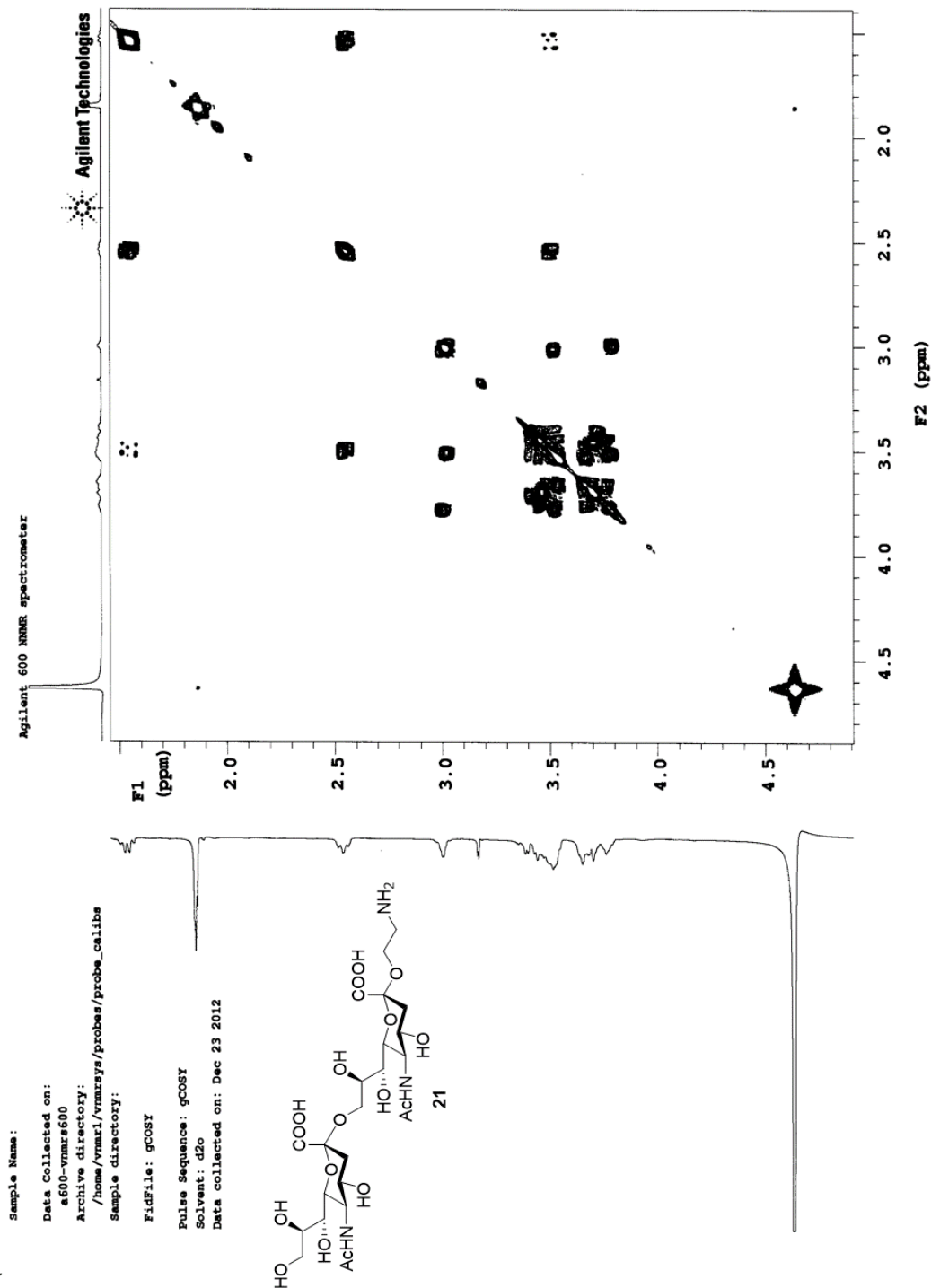
^1\text{H} - ^1\text{H} COSY Spectrum of compound 15 ( \text{D}_2\text{O} , 600 MHz)
