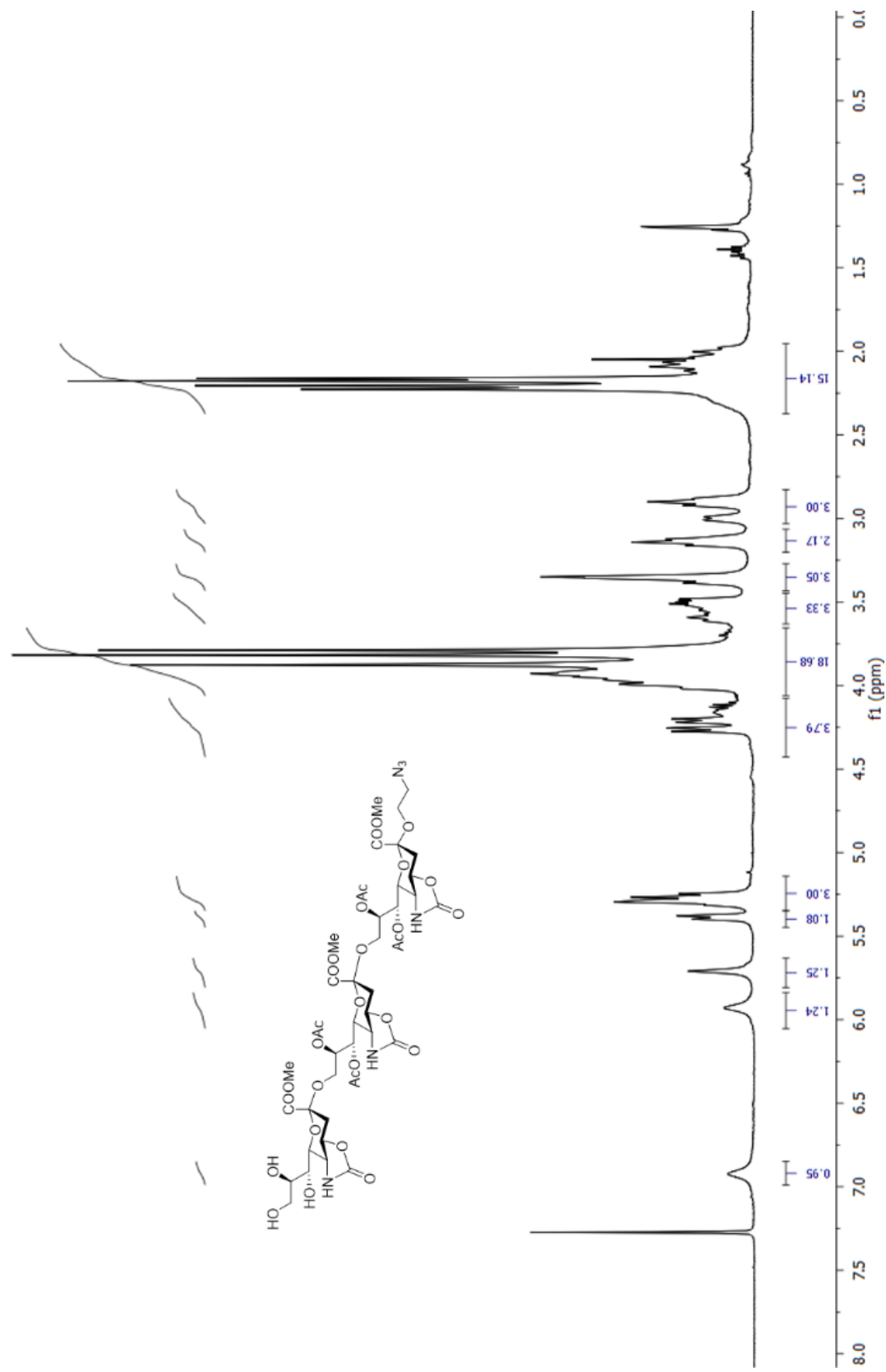
^1\text{H} NMR Spectrum of compound 16 ( \text{CDCl}_3 , 500 MHz)
