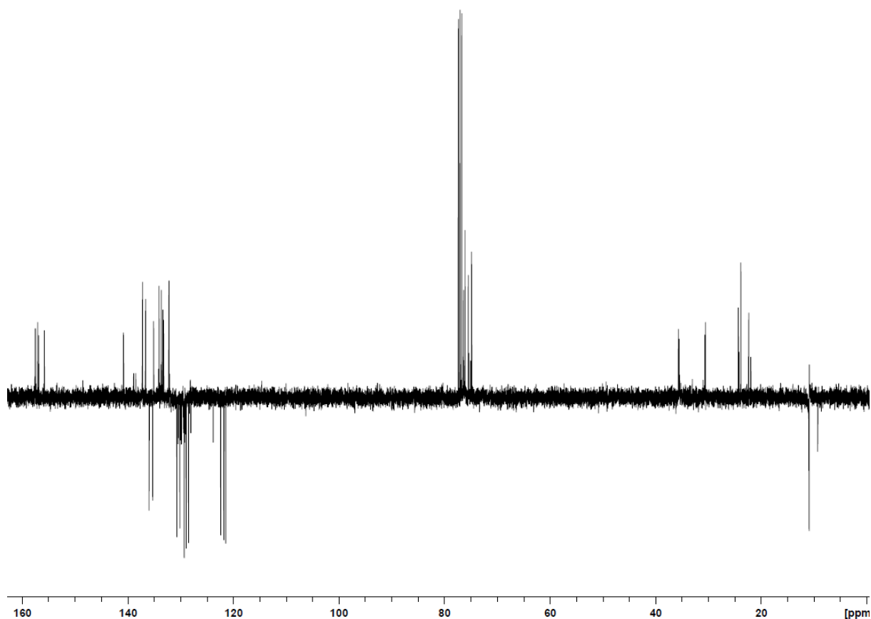
Figure 6. ^{13}\text{C} NMR of compound 2e ( \text{CDCl}_3 , 100 MHz).
