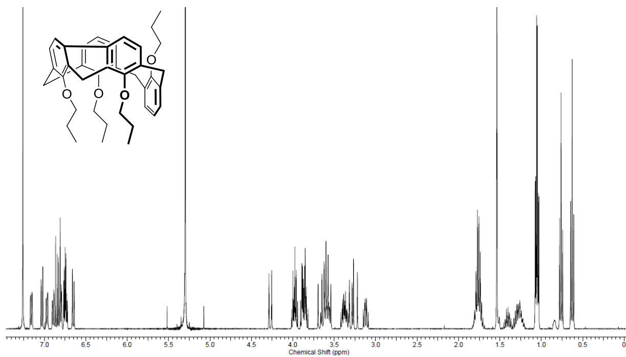
Figure 9. ^1\text{H} NMR of compound 3 ( \text{CDCl}_3 , 300 MHz).
