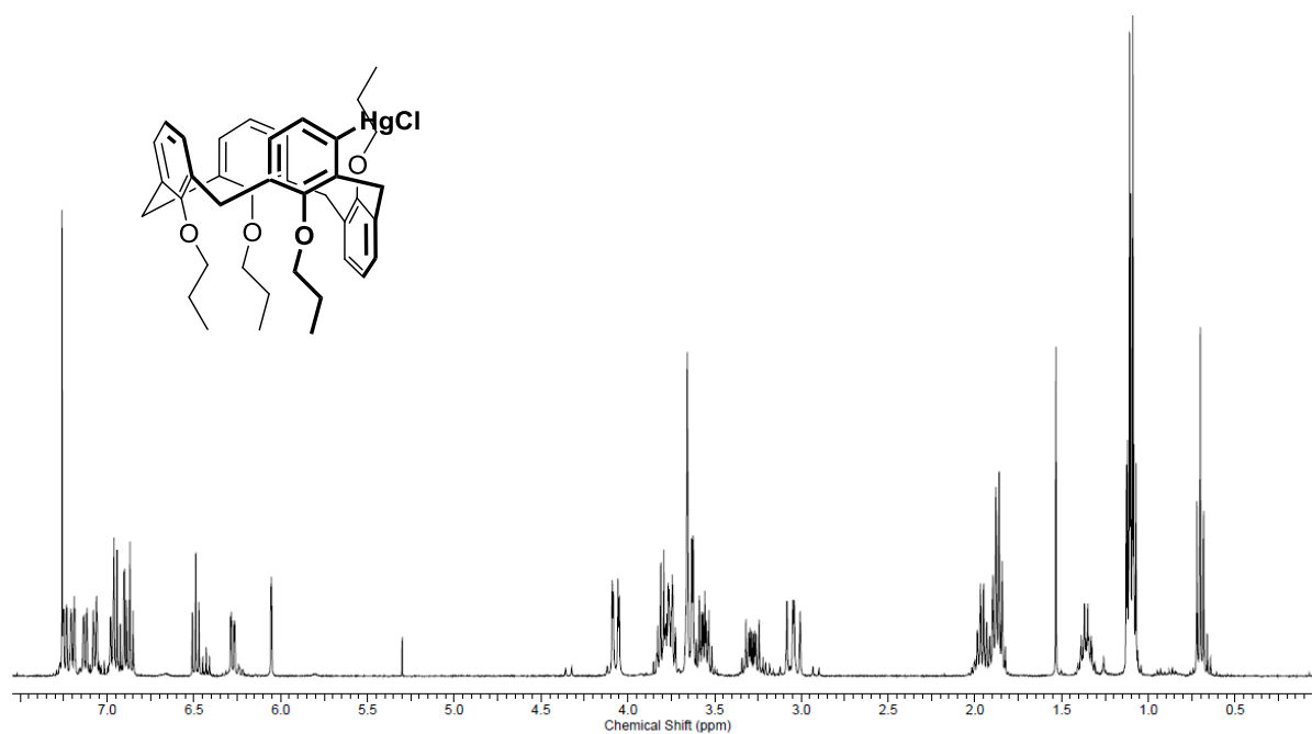
Figure 5. ^1\text{H} NMR of compound 2e ( \text{CDCl}_3 , 400 MHz).
