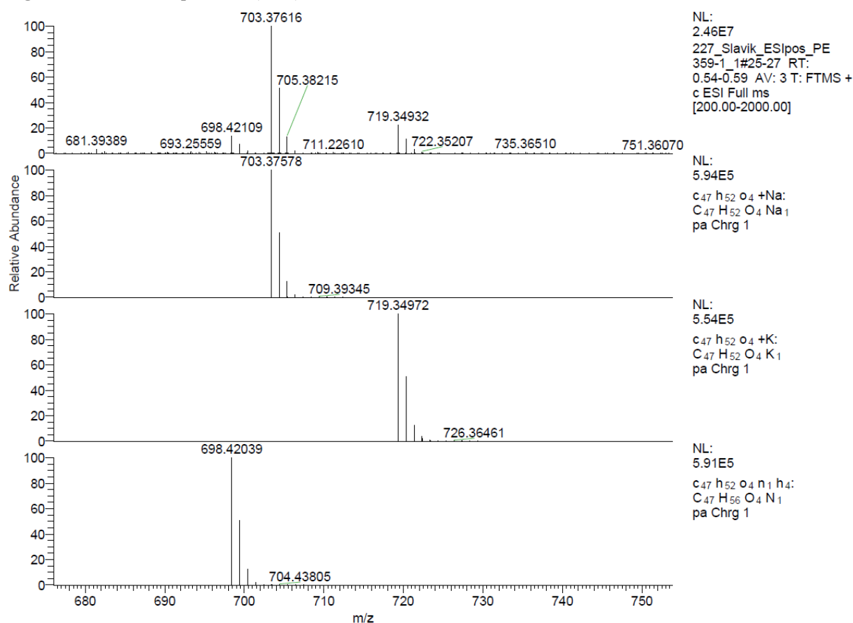
Figure 16. HRMS of compound 4 (ESI + ).
