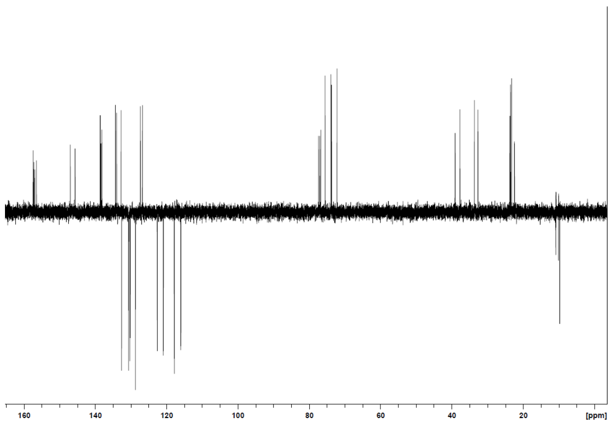
Figure 10. ^{13}\text{C} NMR of compound 3 ( \text{CDCl}_3 , 75 MHz).
