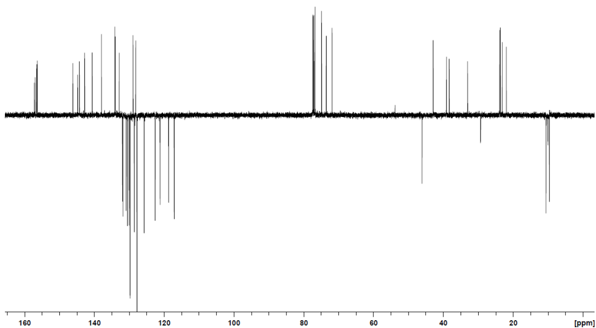
Figure 14. ^{13}\text{C} NMR of compound 4 ( \text{CDCl}_3 , 100 MHz).
