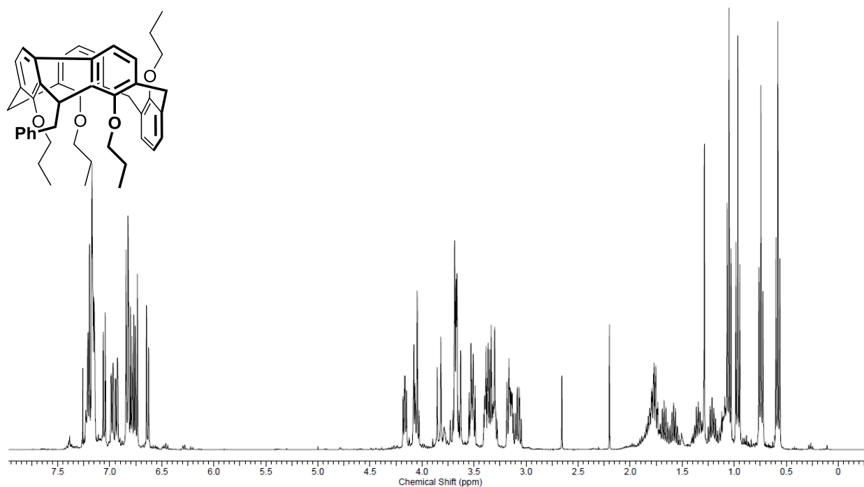
Figure 13. ^1\text{H} NMR of compound 4 ( \text{CDCl}_3 , 400 MHz).
