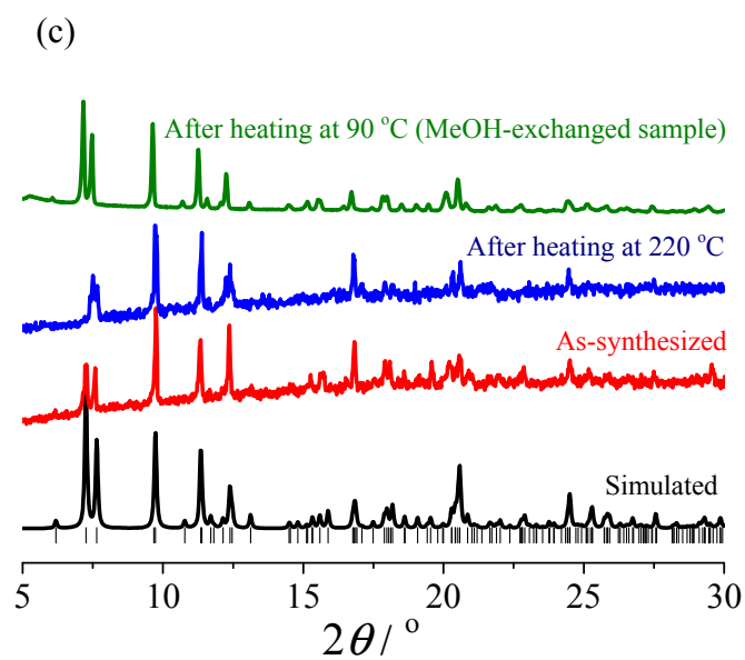
Fig. S2 PXR D patterns of (a)1, (b)2 and (c)3.
