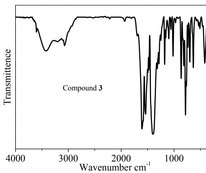
Fig. S1 IR spectra of compounds 1–3.
