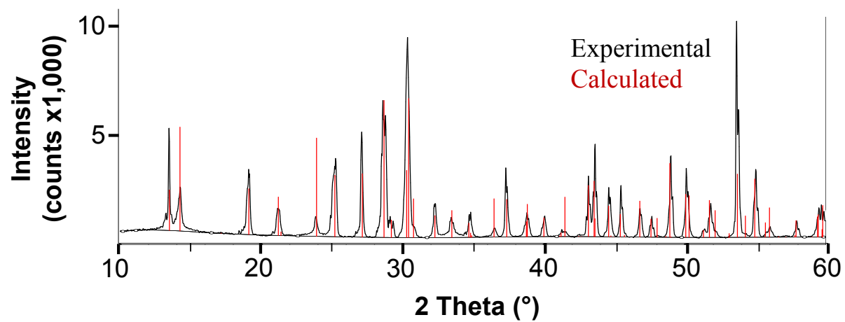
Figure S1. Powder X-ray diffraction pattern of K_4CaUSi_4O_{14} with calculated pattern shown in red.
