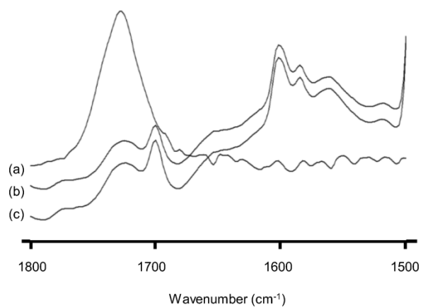
Figure S1. Carbonyl spectral region for (a) HPMCP and HPMC with (b) 30% ATP(S) and (c) 30% ATP(R)
