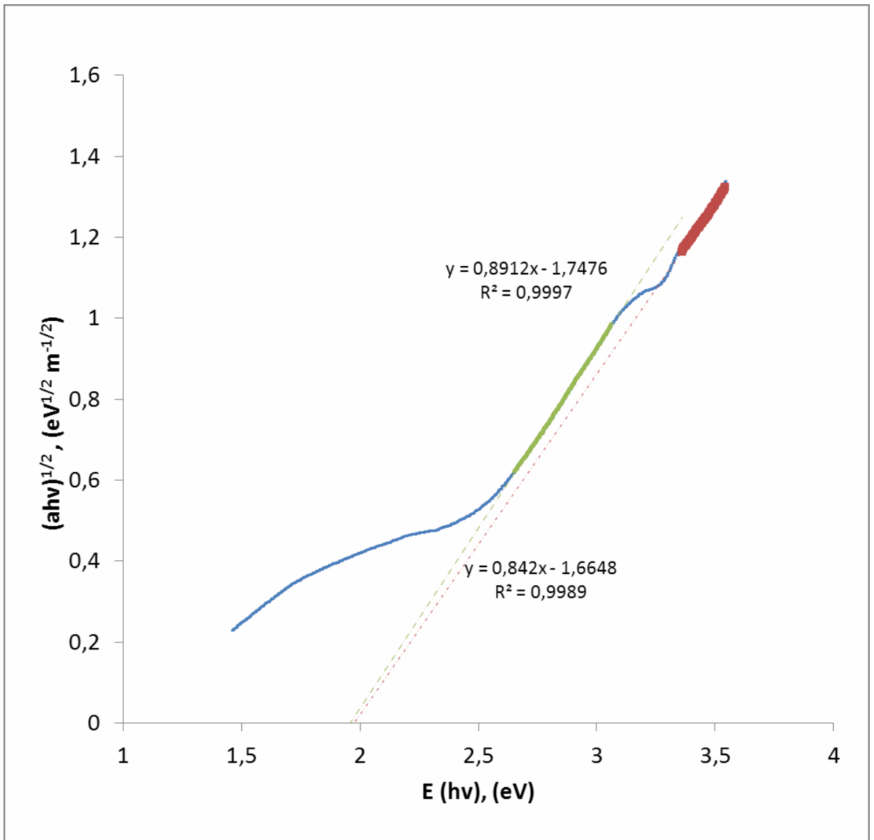
Determination of E_g for sample 11 .
