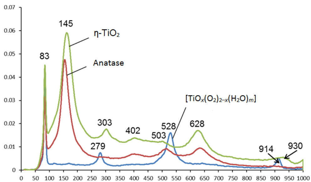
Raman spectra of anatase, \eta\text{-TiO}_2 and [\text{TiO}_x(\text{O}_2)_{2-x}(\text{H}_2\text{O})_m] .
