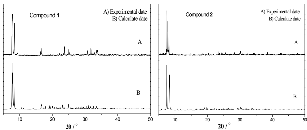
Fig.S3. XRD patterns of compounds 1 and 2.
