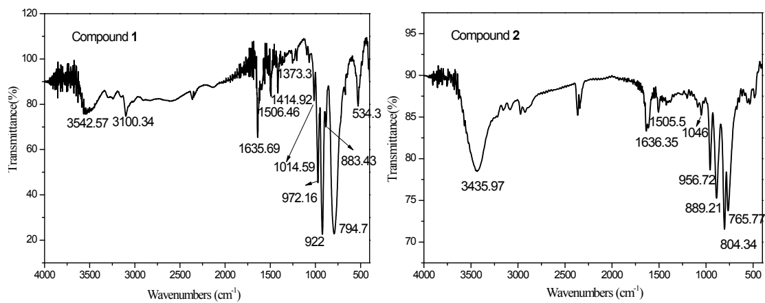
Fig.S2. IR spectra of compounds 1 and 2.
