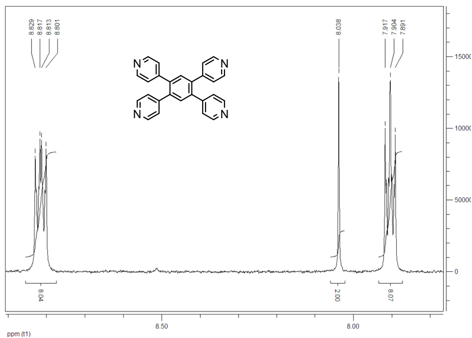
Fig.S1. 1 H NMR spectrum (400 MHz, [D 6 ]DMSO).
