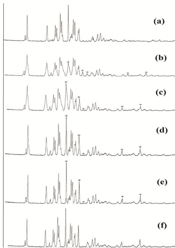
Figure S3 From bottom to top: PXRD pattern of GL-MA (1:1) (f) physical mixture (e) after 1 min grinding (d) after 10 min grinding (c) after 20 min grinding (b) after 40 min grinding (a) after 60 min grinding
