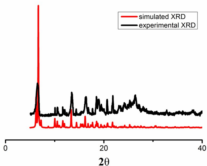
Fig. S2. The simulated PXRD pattern from single crystal data and the experimental PXRD pattern from the crystal samples.
