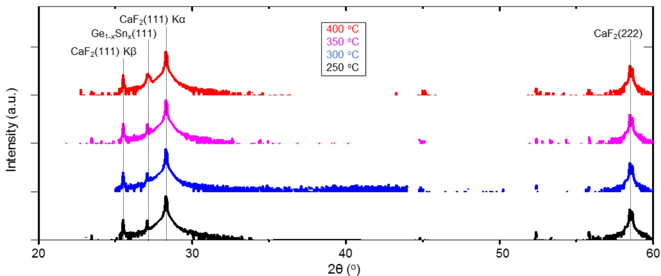
Figure S1. XRD \theta/2\theta scans of \text{Ge}_{1-x}\text{Sn}_x films grown on \text{CaF}_2(111) substrates. Scans are plotted in log scale.
