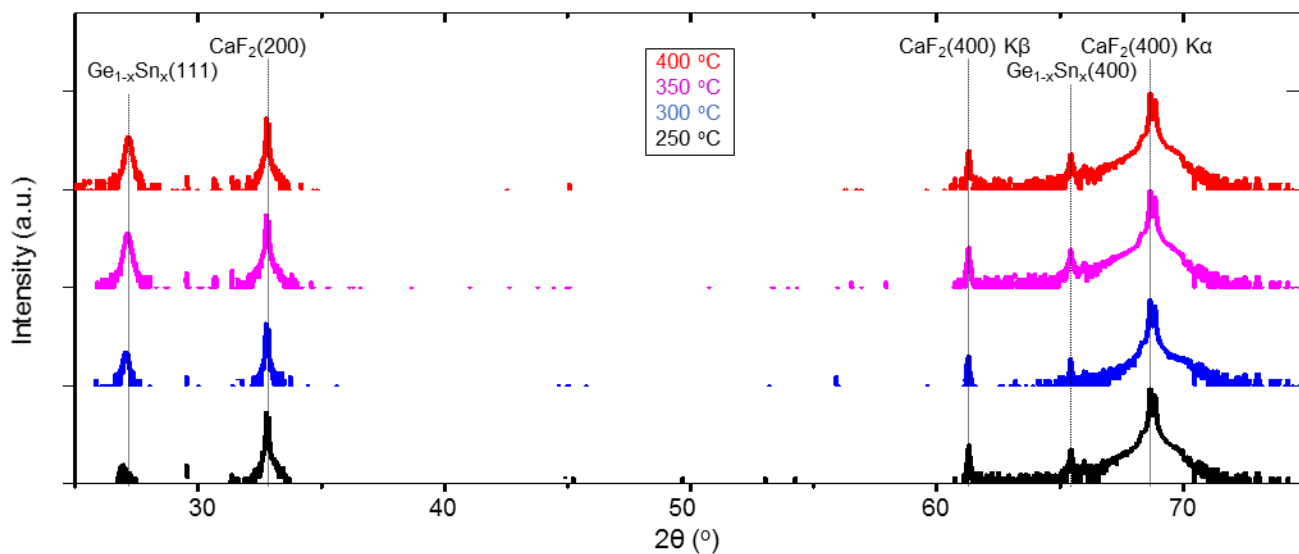
Figure S2. XRD \theta/2\theta scans of \text{Ge}_{1-x}\text{Sn}_x films grown on \text{CaF}_2(100) substrates. Scans are plotted in log scale.
