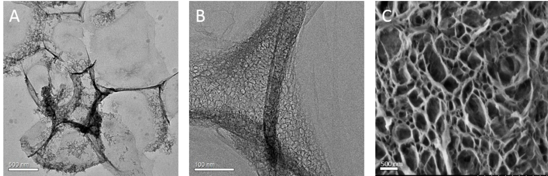
Figure S1 , TEM (A, B) and FESEM (C) images of self-assembled porous foams with mesoporous silica framework by replacing the water with 0.3 mol/L \text{Na}_2\text{SO}_4 aqueous solution while maintaining other conditions.
