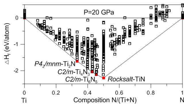
Fig. 6s (Color online). Convex hull diagram of the Ti-N system at 20 GPa.
