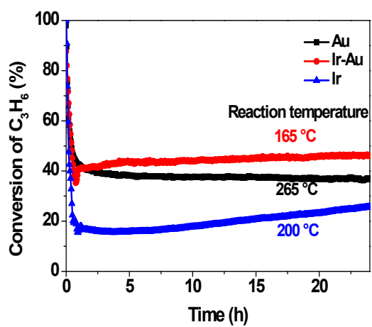
Fig. 1S Evolution of conversion of propene as a function of time on stream of reaction mixture over monometallic Au/TiO 2 , Ir/TiO 2 and bimetallic Ir-Au/TiO 2 samples activated at 400 °C under H 2 .
