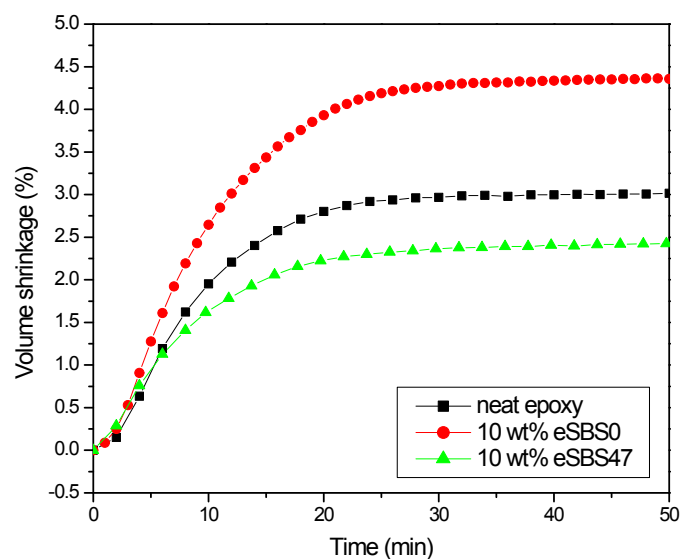
S2. Influence of eSBS (0 and 47) content on the volume shrinkage during curing (initial stages)
