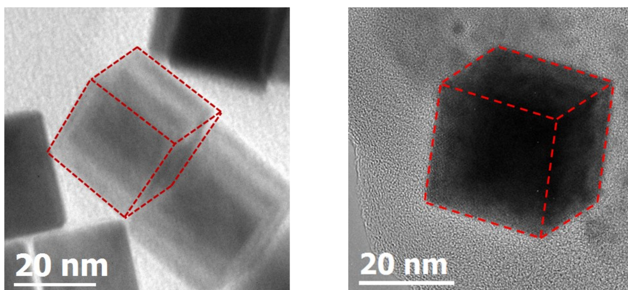
Figure S1: TEM images of the AuCu 3 NPs synthesized by the polyol method revealing the cubic morphology of the as-synthesized particles. The cube edges are highlighted by broken red lines.
