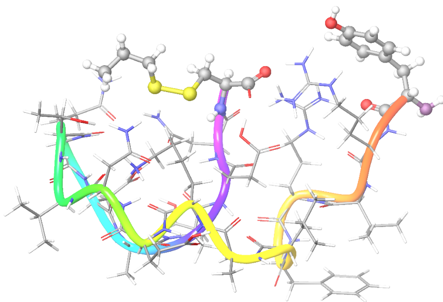
Figure 2: CD36 93-110 2+ LES (R 2 R 4 K 8 C term )
