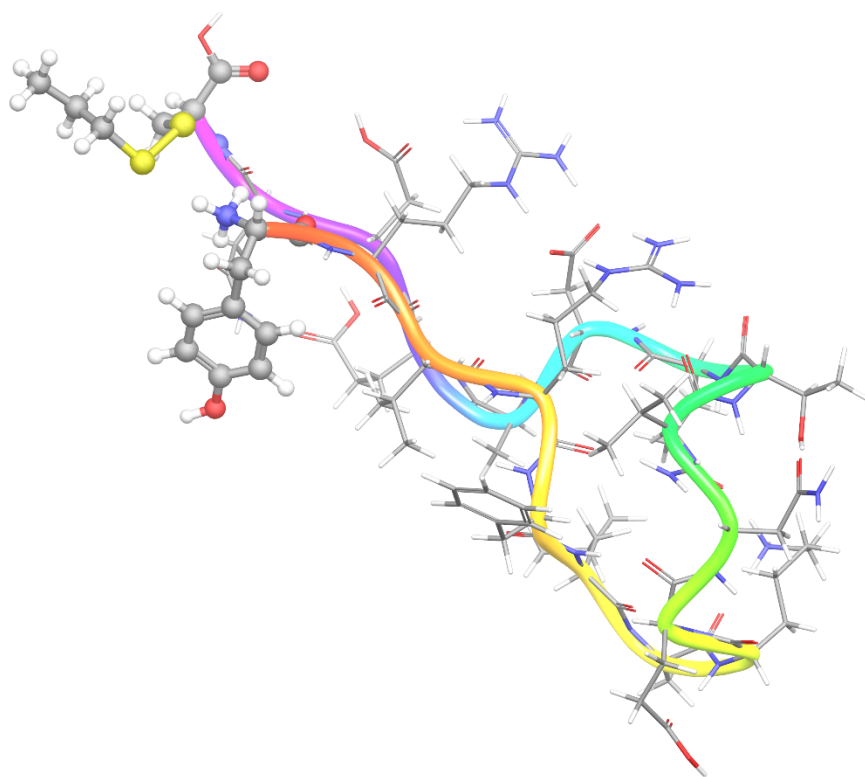
Figure 3: CD36 93-110 3+ (N term R 2 R 4 K 8 D 15 ) structure from constrained simulated annealing.
