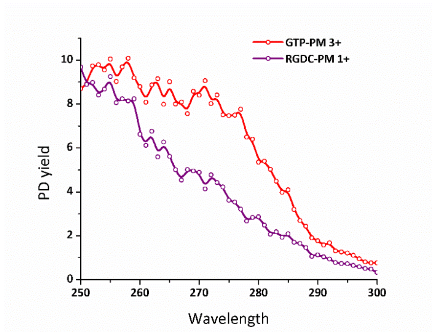
Figure 1: Action-EET spectra of GTP-PM 3+ and RGDC-PM 1+ for comparison
