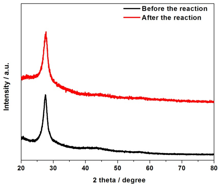
Fig. S2. The XRD patterns of the e-C 3 N 4 /NiS-1.0 before and after the photocatalytic reaction.
