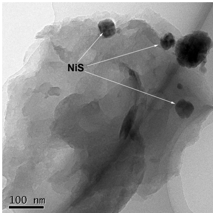
Fig. S1. The TEM image of the used photocatalyst e-C 3 N 4 /NiS-1.0.
