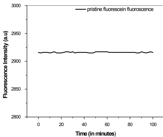
Figure S3. Temporal variation of fluorescence intensity fluorescein under 442 nm excitation
