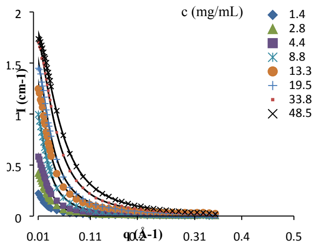
Figure S1. SANS patterns for d-PEO-[Li(G4)]TFSI solutions with background subtracted.
