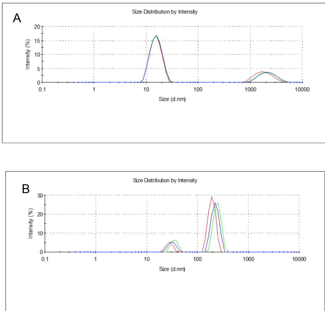
Size distribution curves obtained from DLS at 25°C for A) bicellar systems incorporating \beta -carotene and B) bicosomes incorporating \beta -carotene.
