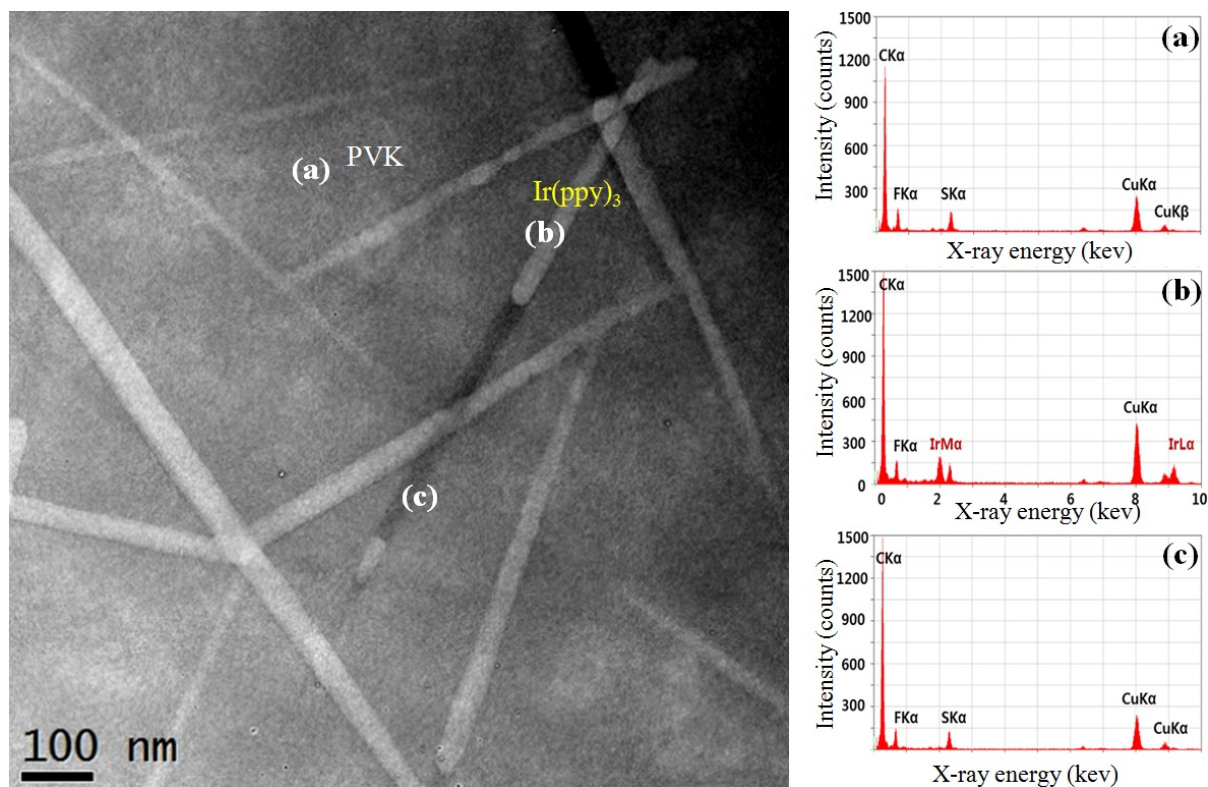
Fig. S1. (S)TEM-HAADF image taken from a thermally annealed PVK:Ir(ppy) 3 at 150 °C showing the local contrast change of the needle-like features and the corresponding EDS results acquired from (a) PVK, (b) and (c) needle-like features, respectively.
