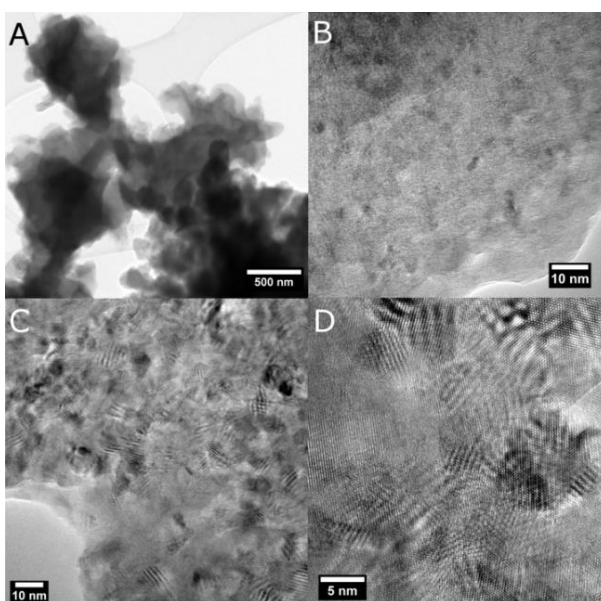
Figure S2. TEM micrographs of Ca-RHC after the first desorption displaying A) large aggregates of smaller particles, B) multiphase regions of low crystallinity C) and D) multiphase region of high crystallinity.
