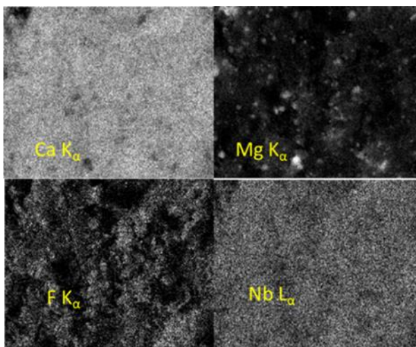
Figure S1. Elemental maps obtained by EDS for the NbF 5 doped Ca-RHC sample after desorption.
