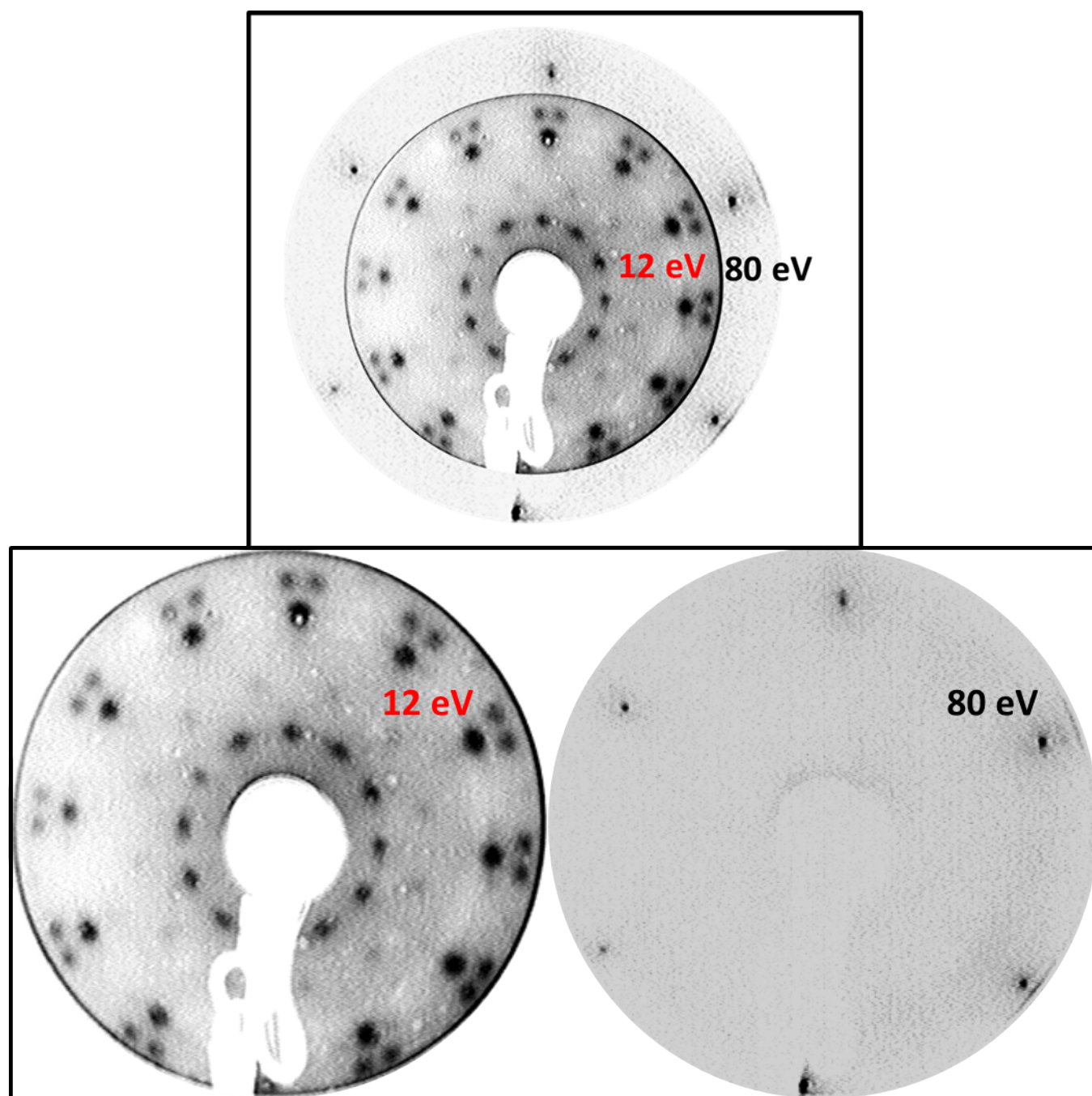
Figure S1 – Nested LEED patterns (upper panel) of a clean Au (111) surface (outer, 80 eV) and 1 ML VOPc / Au (111) (inner, 12 eV), each pattern is reproduced individually in the lower panel.
