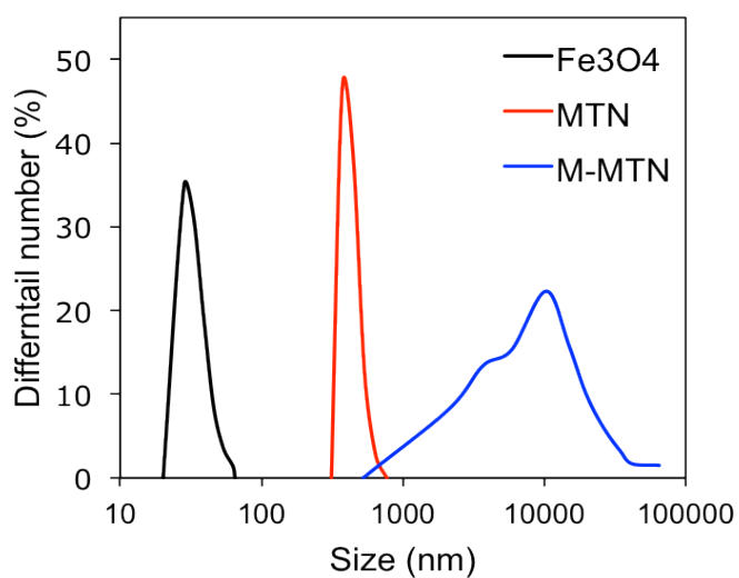
Figure S1. Particle size distribution of Fe 3 O 4 , MTN, and M-MTN.
