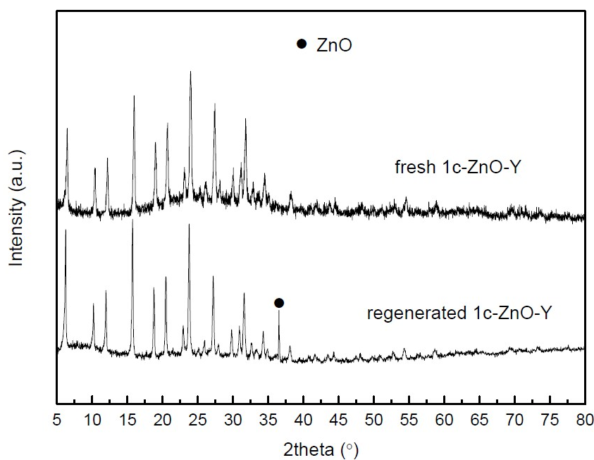
Figure S1. XRD patterns of fresh and regenerated 1c-ZnO-Y catalysts
