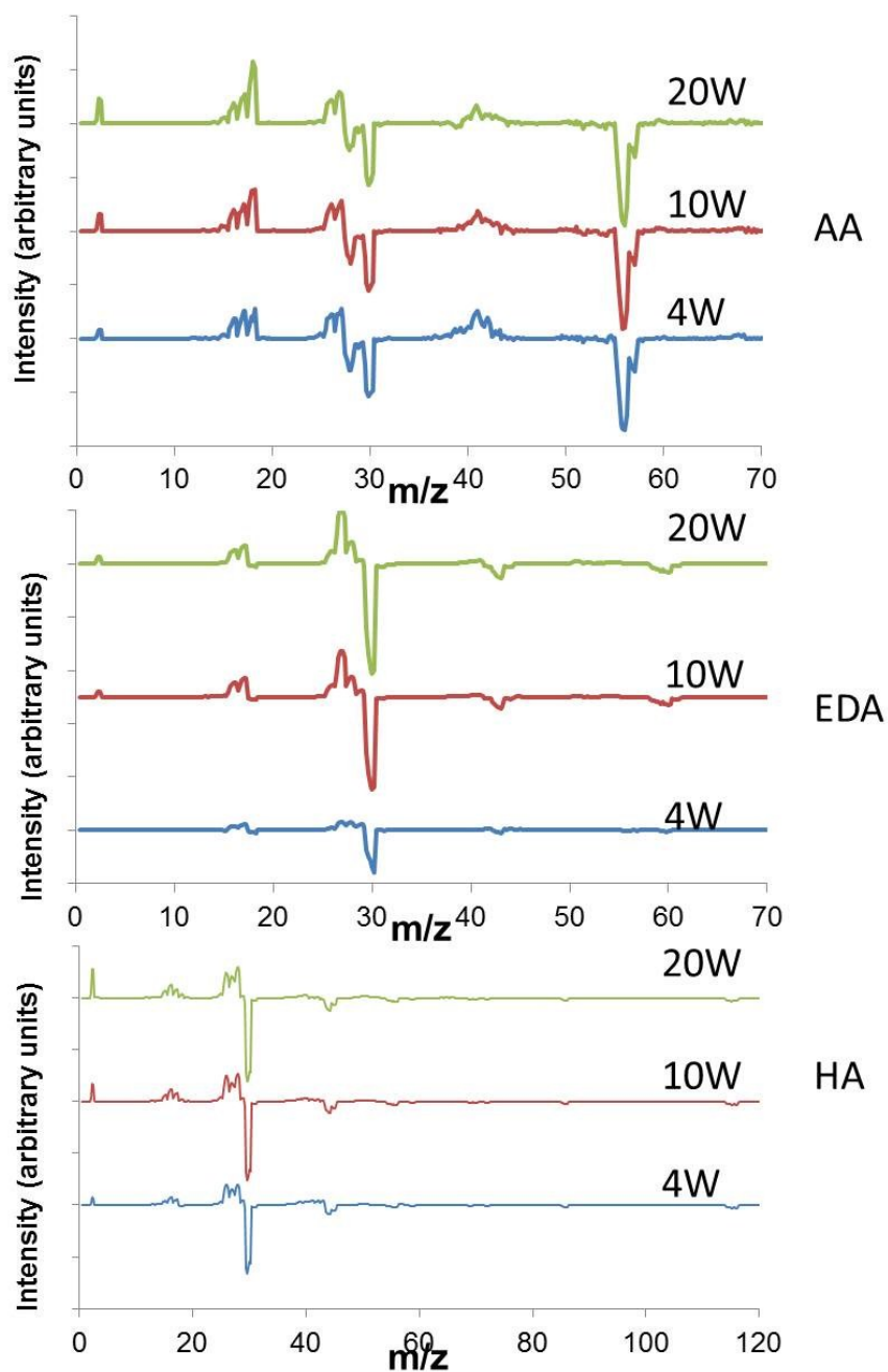
Figure S1. Change in neutral species distribution with applied power for AA (top), EDA (middle) and HA (bottom) compared to electron impact with no plasma.
