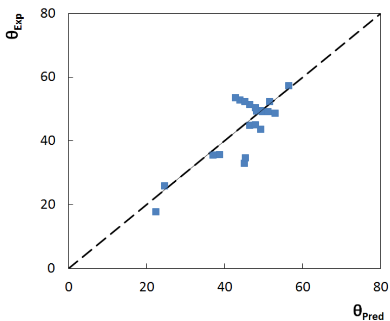
Figure S20. Comparison between experimental, \theta_{\text{Exp}} , and predictive, \theta_{\text{Pred}} , contact angles values using Equation S18.
