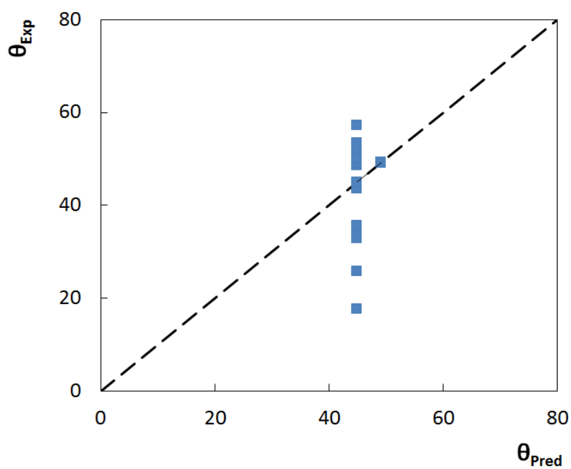
Figure S16. Comparison between experimental, \theta_{\text{Exp}} , and predictive, \theta_{\text{Pred}} , contact angles values using Equation S14.
