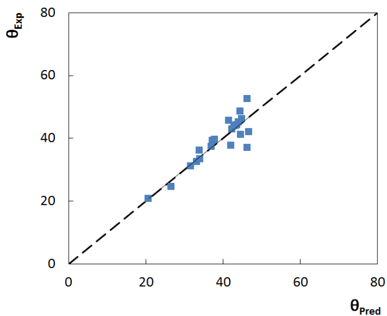
Figure S6. Comparison between experimental, \theta_{\text{Exp}} , and predictive, \theta_{\text{Pred}} , contact angles values using Equation S5.
