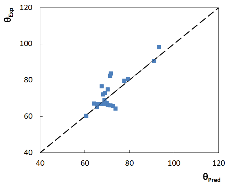
Figure S23. Comparison between experimental, \theta_{\text{Exp}} , and predictive, \theta_{\text{Pred}} , contact angles values using Equation S21.
