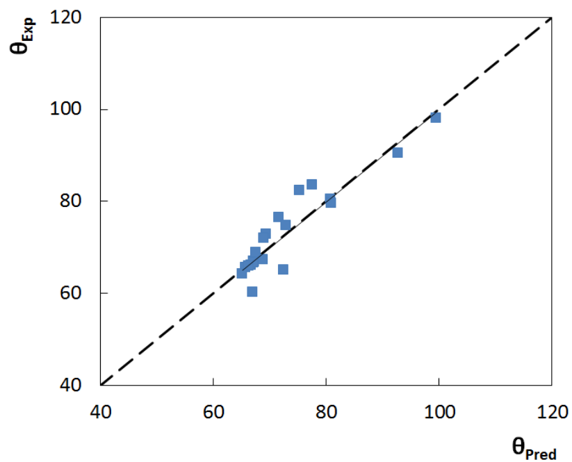
Figure S30. Comparison between experimental, \theta_{\text{Exp}} , and predictive, \theta_{\text{Pred}} , contact angles values using Equation S27.
