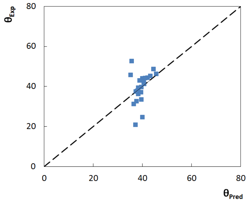
Figure S3. Comparison between experimental, \theta_{\text{Exp}} , and predictive, \theta_{\text{Pred}} , contact angles values using Equation S2.
