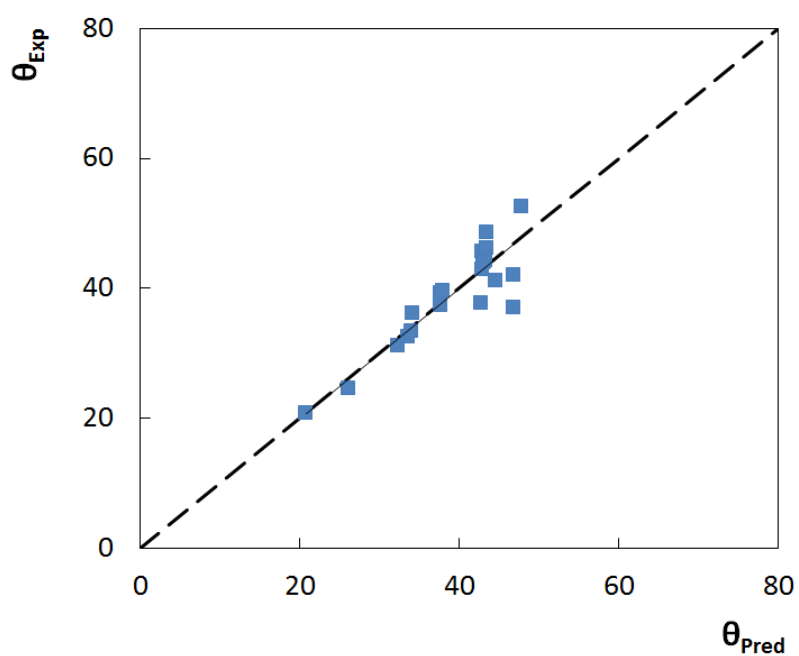
Figure S2. Comparison between experimental, \theta_{\text{Exp}} , and predictive, \theta_{\text{Pred}} , contact angles values using Equation 3.
