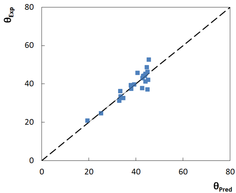
Figure S11. Comparison between experimental, \theta_{\text{Exp}} , and predictive, \theta_{\text{Pred}} , contact angles values using Equation S10.
