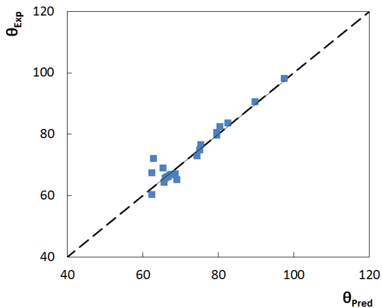
Figure S29. Comparison between experimental, \theta_{\text{Exp}} , and predictive, \theta_{\text{Pred}} , contact angles values using Equation S26.
