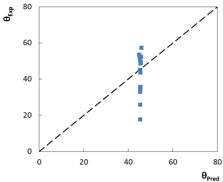
Figure S15. Comparison between experimental, \theta_{\text{Exp}} , and predictive, \theta_{\text{Pred}} , contact angles values using Equation S13.
