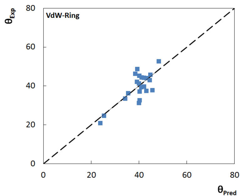
Figure S10. Comparison between experimental, \theta_{\text{Exp}} , and predictive, \theta_{\text{Pred}} , contact angles values using Equation S9.
