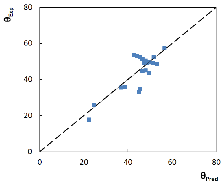
Figure S12. Comparison between experimental, \theta_{\text{Exp}} , and predictive, \theta_{\text{Pred}} , contact angles values using Equation S11.
