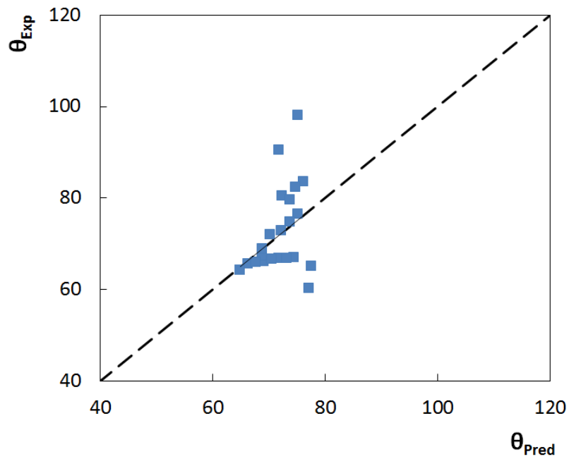
Figure S32. Comparison between experimental, \theta_{\text{Exp}} , and predictive, \theta_{\text{Pred}} , contact angles values using Equation S29.
