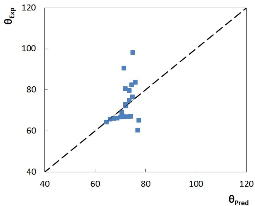
Figure S25. Comparison between experimental, \theta_{\text{Exp}} , and predictive, \theta_{\text{Pred}} , contact angles values using Equation S22.
