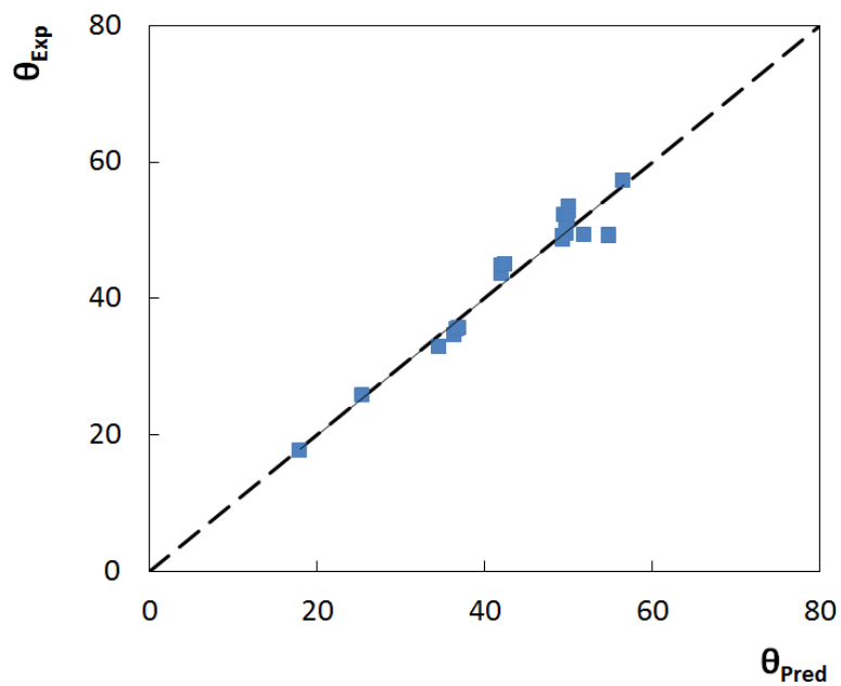
Figure S17. Comparison between experimental, \theta_{\text{Exp}} , and predictive, \theta_{\text{Pred}} , contact angles values using Equation S15.
