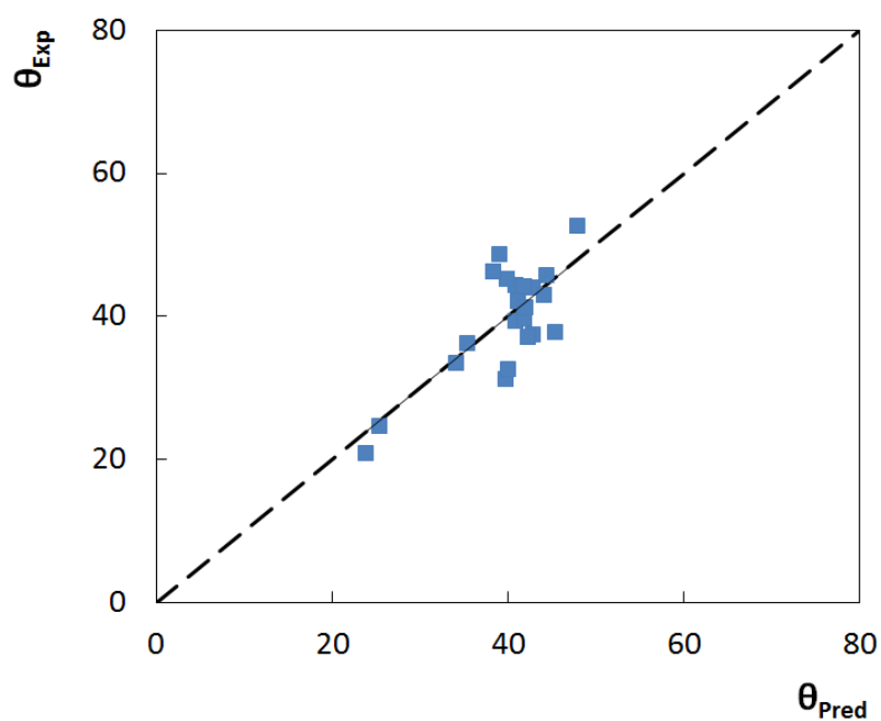
Figure S1. Comparison between experimental, \theta_{\text{Exp}} , and predictive, \theta_{\text{Pred}} , contact angles values using Equation S1.
