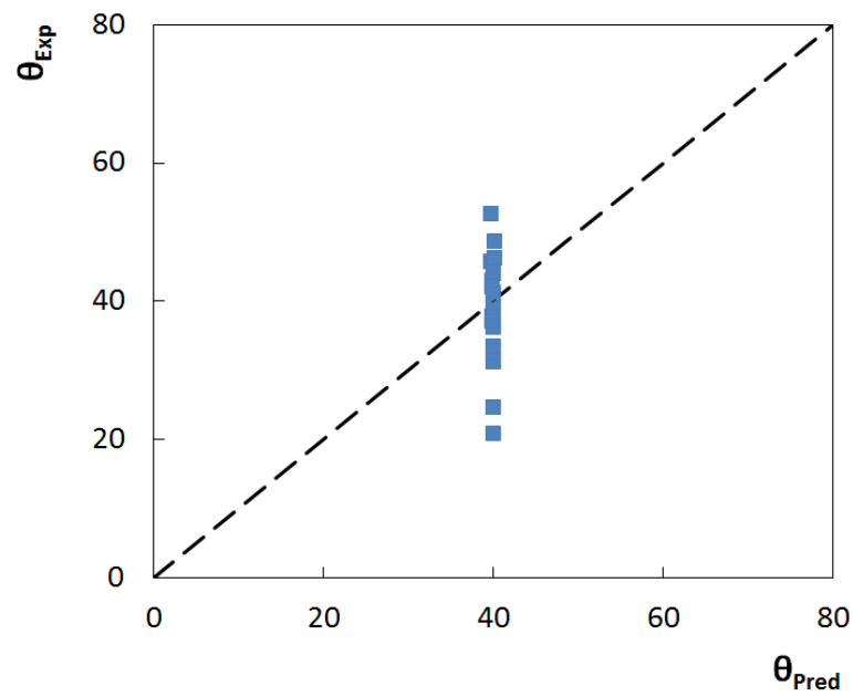
Figure S4. Comparison between experimental, \theta_{\text{Exp}} , and predictive, \theta_{\text{Pred}} , contact angles values using Equation S3.
