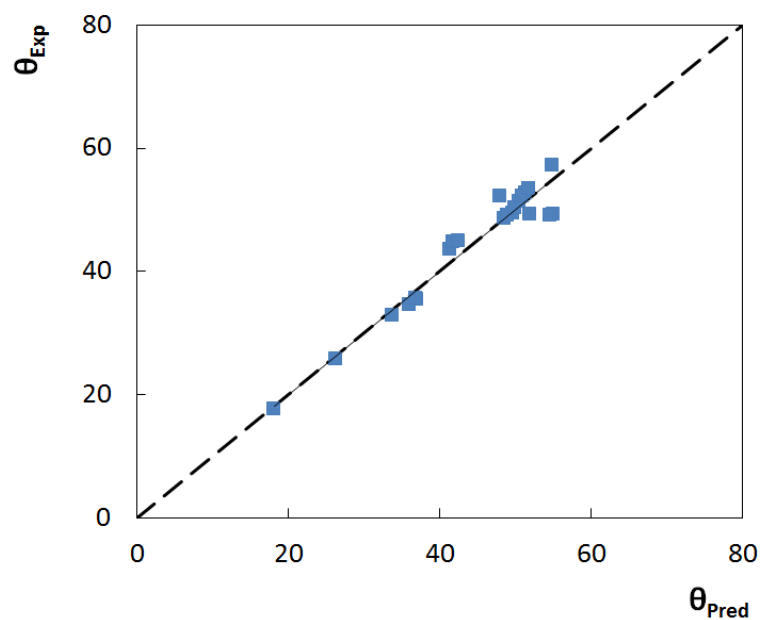
Figure S18. Comparison between experimental, \theta_{\text{Exp}} , and predictive, \theta_{\text{Pred}} , contact angles values using Equation S16.
