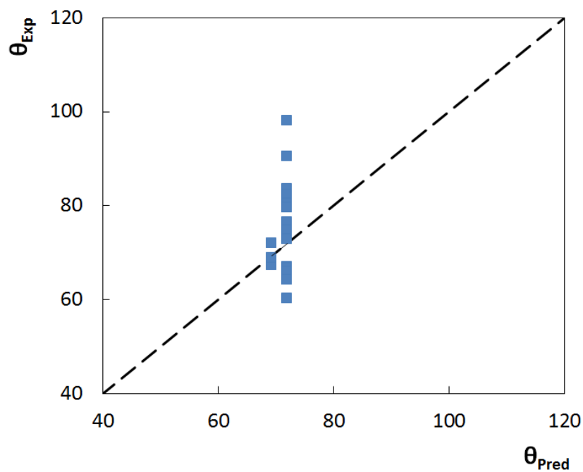
Figure S27. Comparison between experimental, \theta_{\text{Exp}} , and predictive, \theta_{\text{Pred}} , contact angles values using Equation S24.
