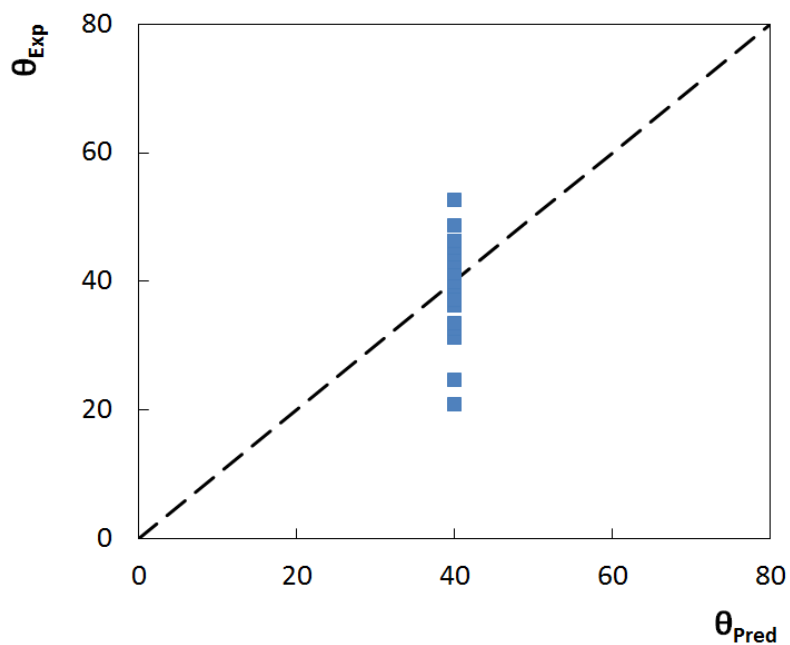
Figure S5. Comparison between experimental, \theta_{\text{Exp}} , and predictive, \theta_{\text{Pred}} , contact angles values using Equation S4.
