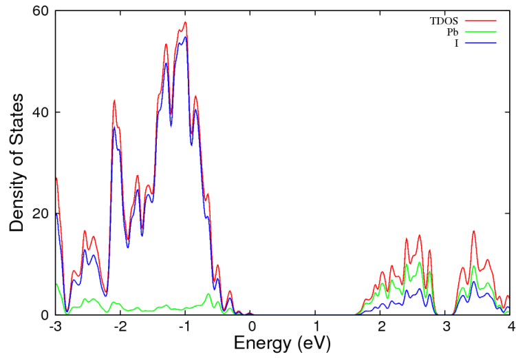
DOS of CH 3 NH 3 PbI 3
