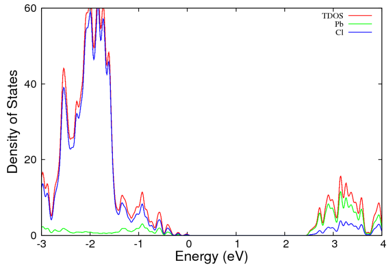
DOS of \text{CH}_3\text{NH}_3\text{PbCl}_3
