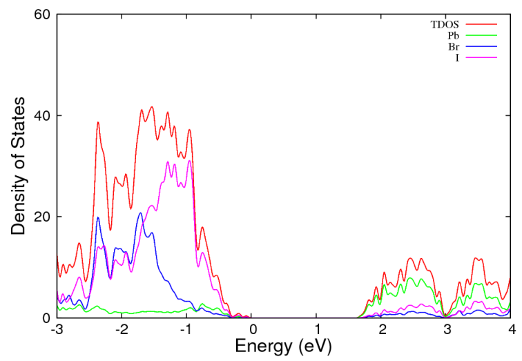
DOS of \text{CH}_3\text{NH}_3\text{PbI}_2\text{Br}
