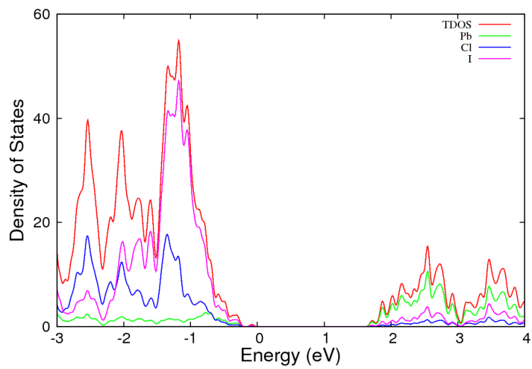
DOS of CH 3 NH 3 PbI 2 Cl
