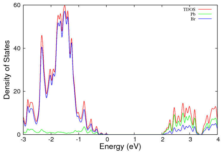
DOS of CH 3 NH 3 PbBr 3
