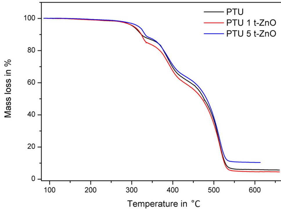
Fig. S2: Thermogravimetric analysis of pure PTU and PTU/t-ZnO composites with varying t-ZnO filling fractions (wt%).
