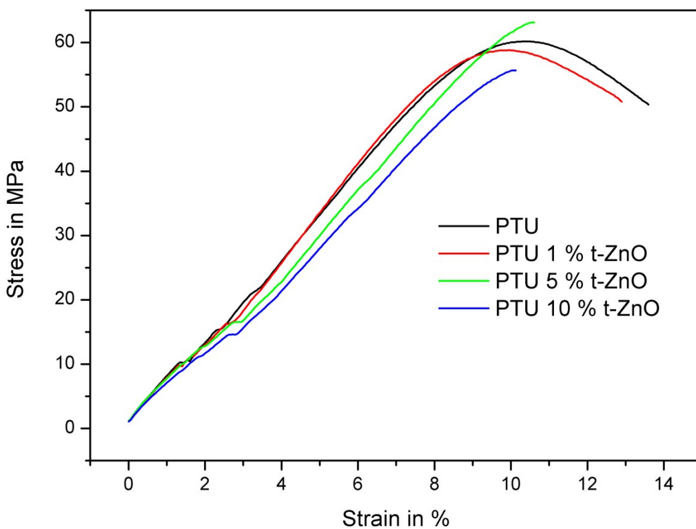
Fig. S1: Stress-strain diagram of pure PTU and PTU/t-ZnO composites with varying t-ZnO filling fractions (wt%).
