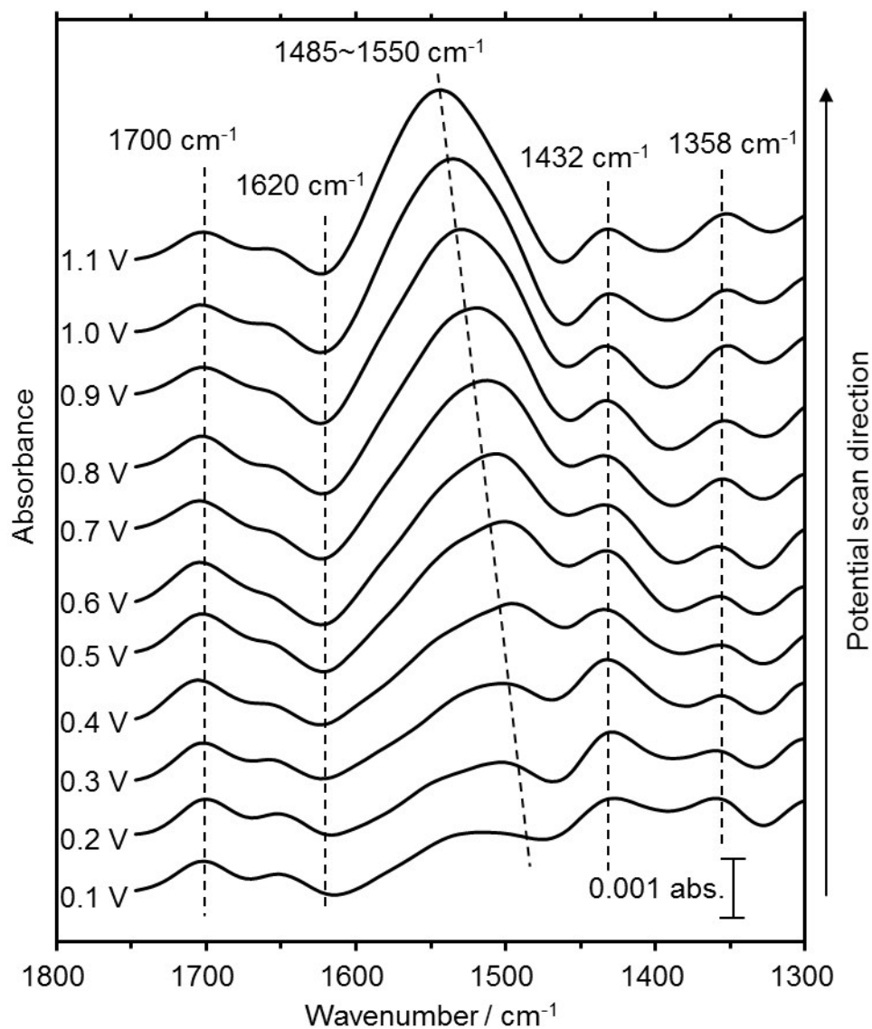
Fig. S1. Time-resolved IR spectra of the Pt surface acquired simultaneously with the linear sweep voltammograms in 0.25 M KOH solution with 1 M ^{13}\text{C} acetone.
