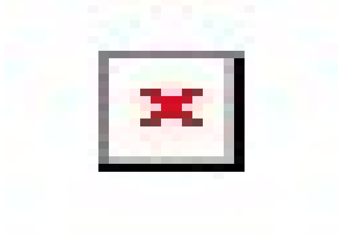
Figure S2. Envelopes of the function L(\mathbf{r})=0.0016 au for F-Br \cdots Br-F complex.
