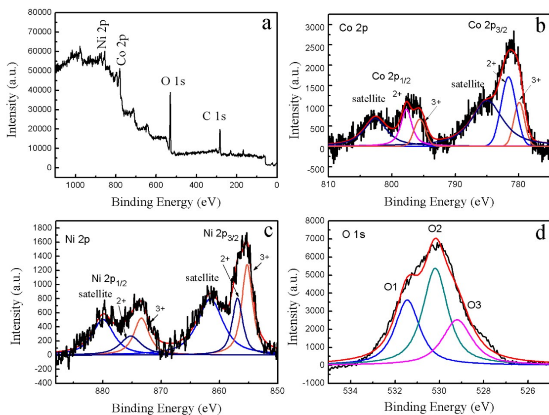
Fig. S1 XPS spectra of (a) full scan survey. (b) Co 2p for NiCo 2 O 4 hollow nanocubes. (c) Ni 2p for NiCo 2 O 4 hollow nanocubes. (d) O 1s for NiCo 2 O 4 hollow nanocubes.
