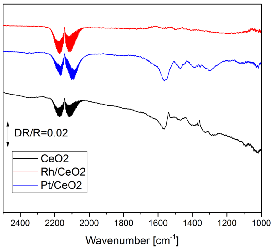
Figure 1: DRIFTS spectra of CeO 2 , Rh/CeO 2 and Pt/CeO 2 after dosing a CO/O 2 mixture at 50 °C
