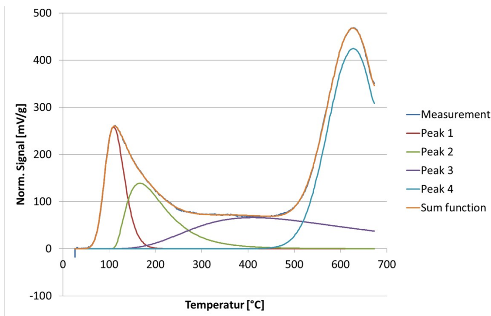
Figure S1. TPD-NH 3 and corresponding spectrum deconvolution of regenerated AlN catalyst after the first run (AlN-R1) (Figure 10 (c)).
