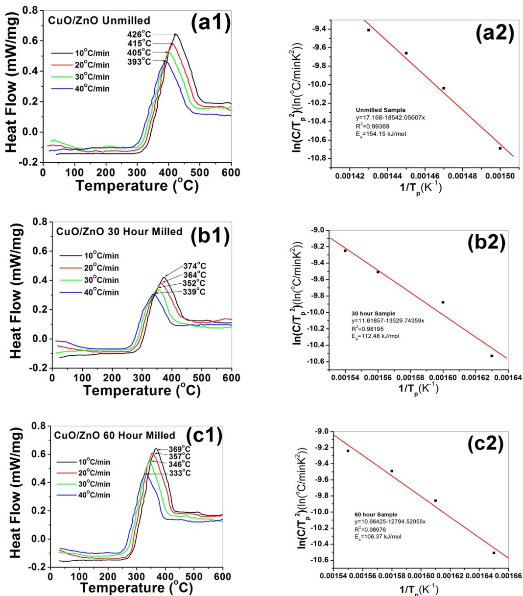
Figures: DSC thermograms for (a1) unmilled (b1) 30 hour milled and (c1) 60 hour milled samples. Kissinger plot for (a2) unmilled (b2) 30 hour milled and (c2) 60 hour milled samples for the determination of activation energy of the three systems.
