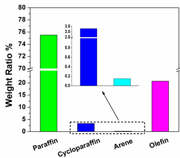
Figure. S2 PONA composition of products of hybrid catalyst: Y-30%: AlPO-11 = 10:1 (wt%)
