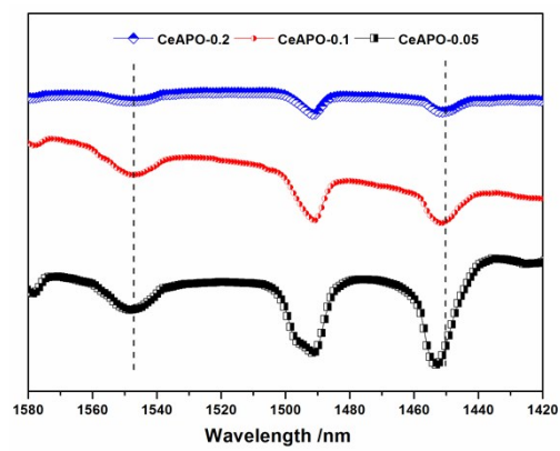
Fig. S1 Py-FTIR spectra of samples
