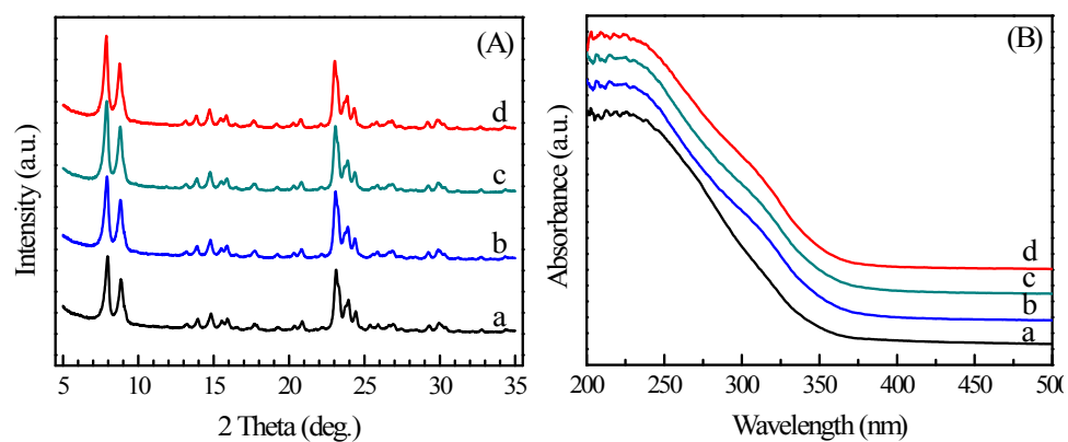
Figure S2. XRD patterns (A), UV-vis spectra (B) of fresh TS-1-MS (a), first regenerated (b), second regenerated (c), and thirdly regenerated (d).
