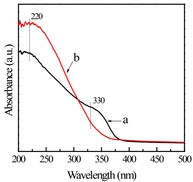
Figure S1. UV-vis spectra of TS-1 (a) and TS-1-MS (b).
