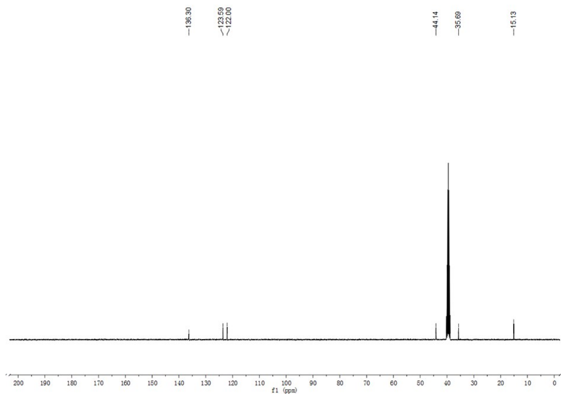
Fig. S4 13 C NMR spectrum of complex 2.
