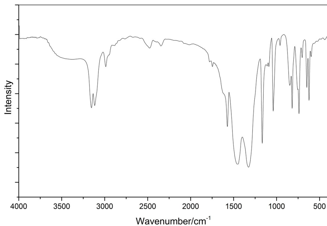
Fig. S12 IR spectrum of complex 2 .
