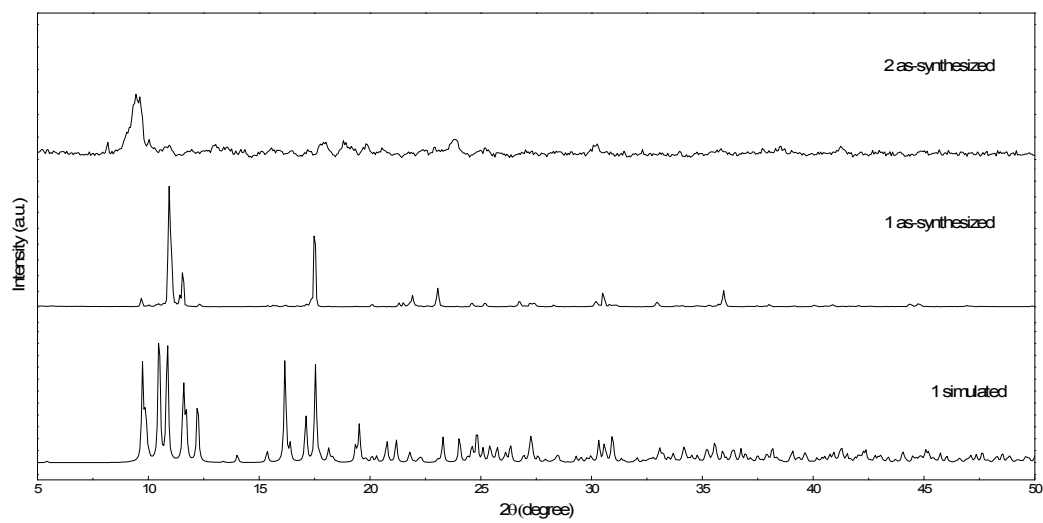
Fig. S16 PXRD spectra of complex 1 and 2 .
