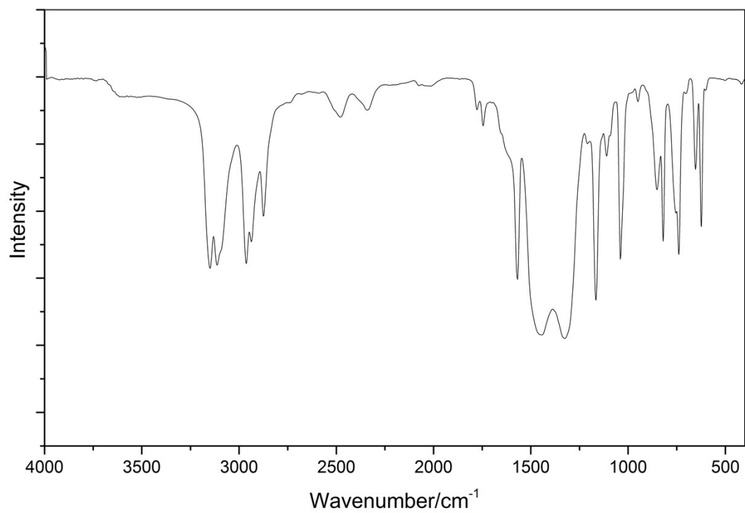
Fig. S13 IR spectrum of complex 3 .
