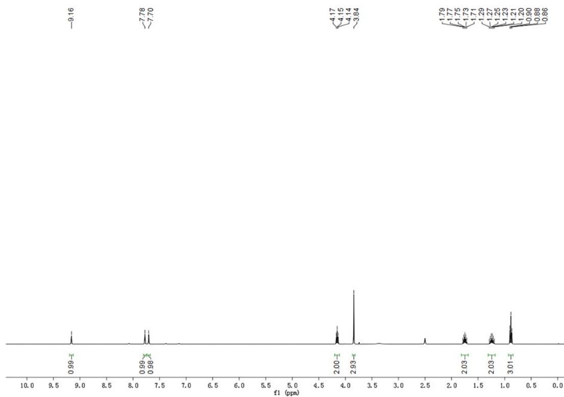
Fig. S5 1 H NMR spectrum of complex 3.
