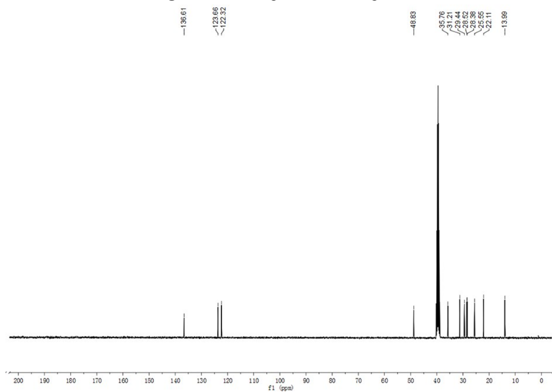
Fig. S10 ^{13}\text{C} NMR spectrum of complex 5 .
