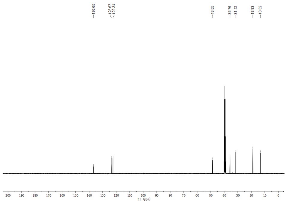
Fig. S6 13 C NMR spectrum of complex 3.
