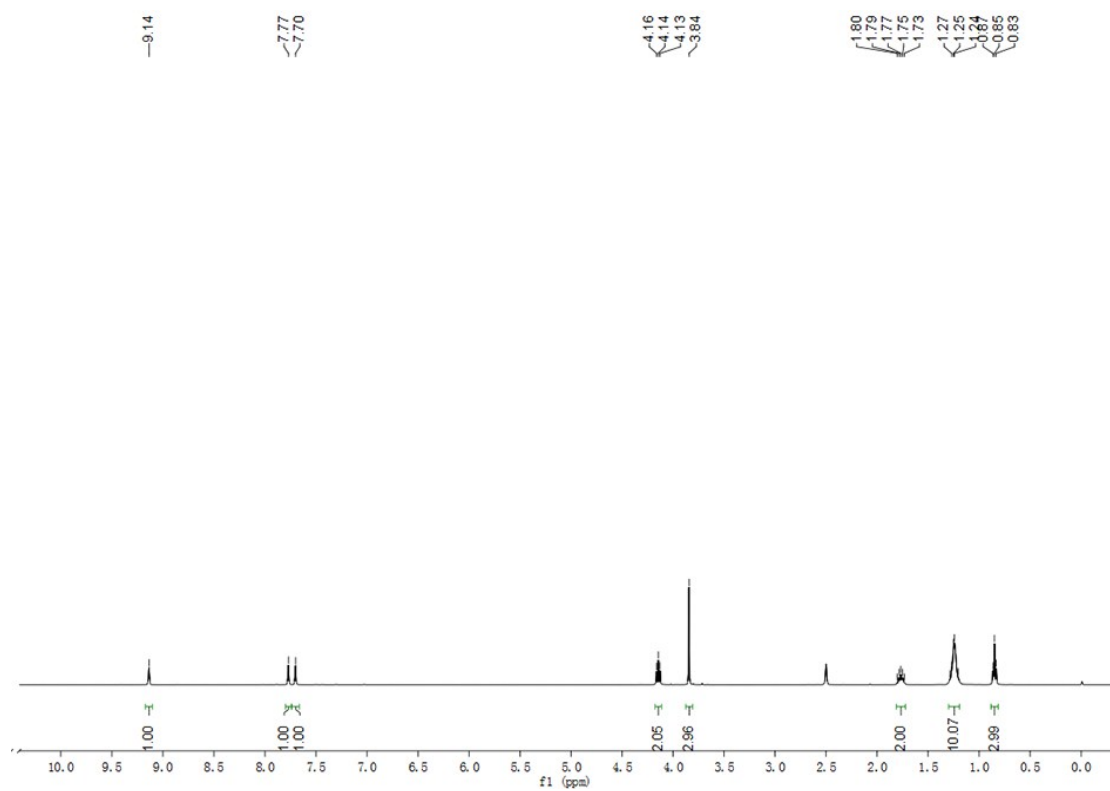
Fig. S9 ^1\text{H} NMR spectrum of complex 5 .
