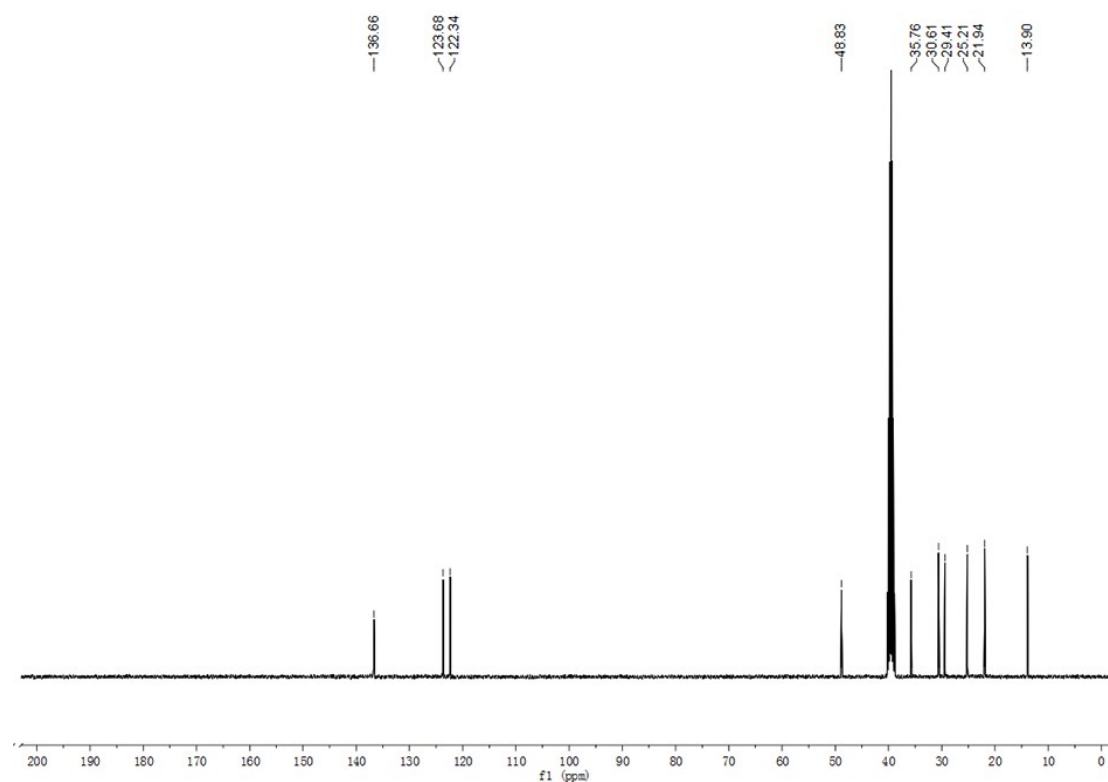
Fig. S8 13 C NMR spectrum of complex 4.
