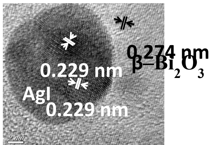
Figure S1 HRTEM image of the 20%-AgI/ \beta - \text{Bi}_2\text{O}_3 composite photocatalyst.
