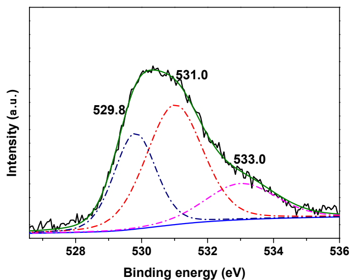
Figure S2 XPS spectra of O1s in the 20%-AgI/ \beta - \text{Bi}_2\text{O}_3 composite photocatalyst.
