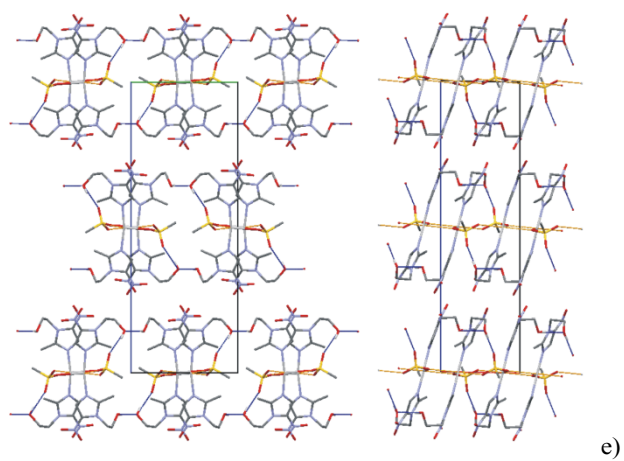
Fig. S2. Crystal packing of 1–5 ( a - e ) along a and b axis, respectively. (C-)H atoms and minor part of disordered atoms (B) have been omitted for clarity.
