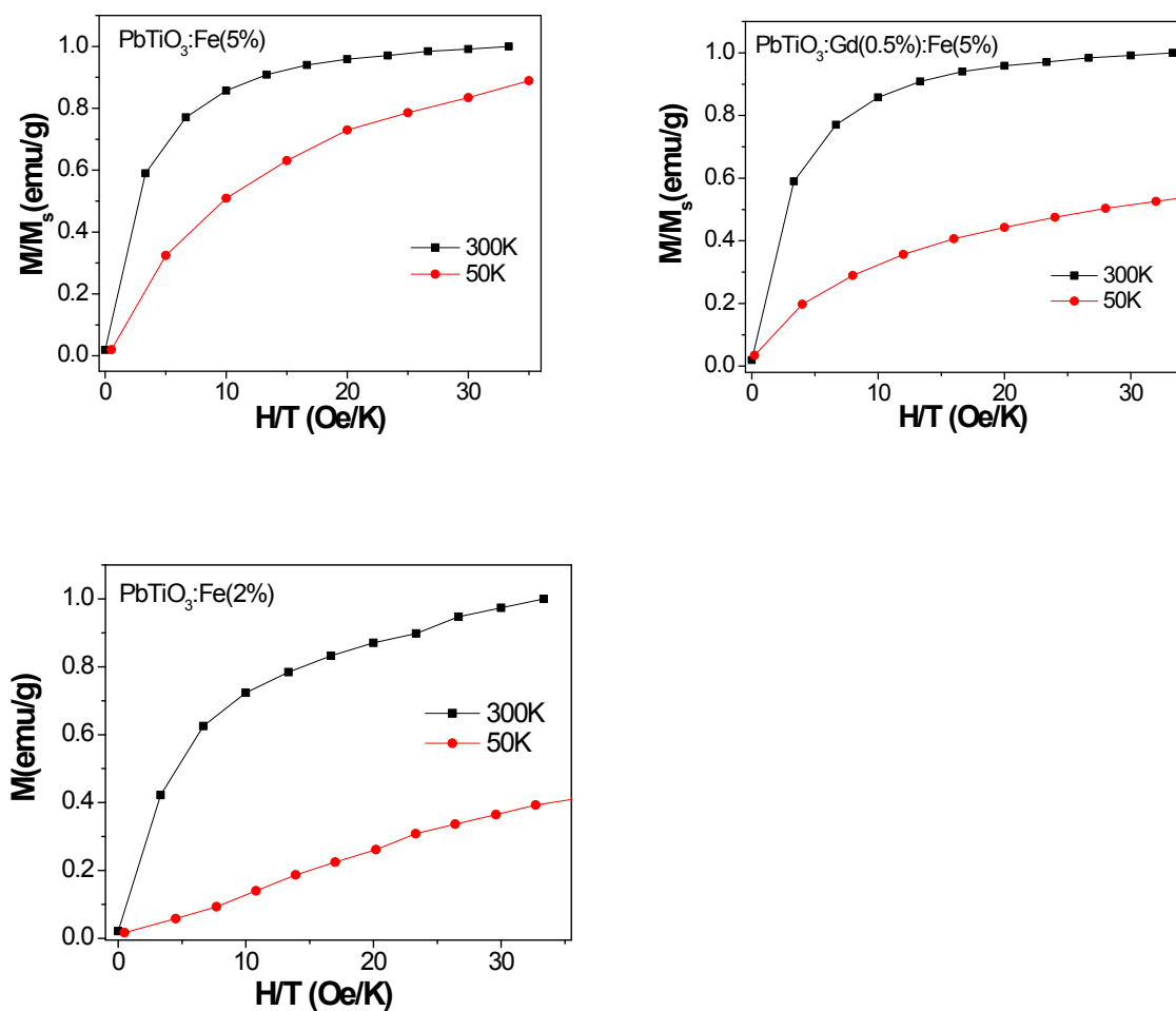
Figure S1: M/M_s vs H/T curves for \text{PbTiO}_3:\text{Fe}(2\%) , \text{PbTiO}_3:\text{Fe}(5\%) and \text{PbTiO}_3:\text{Fe}(5\%):\text{Gd}(0.5\%) samples at 50K and 300K.
