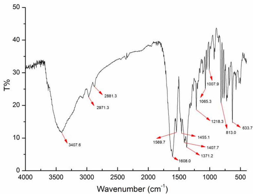
Figure S1. The IR spectra of 1-D
