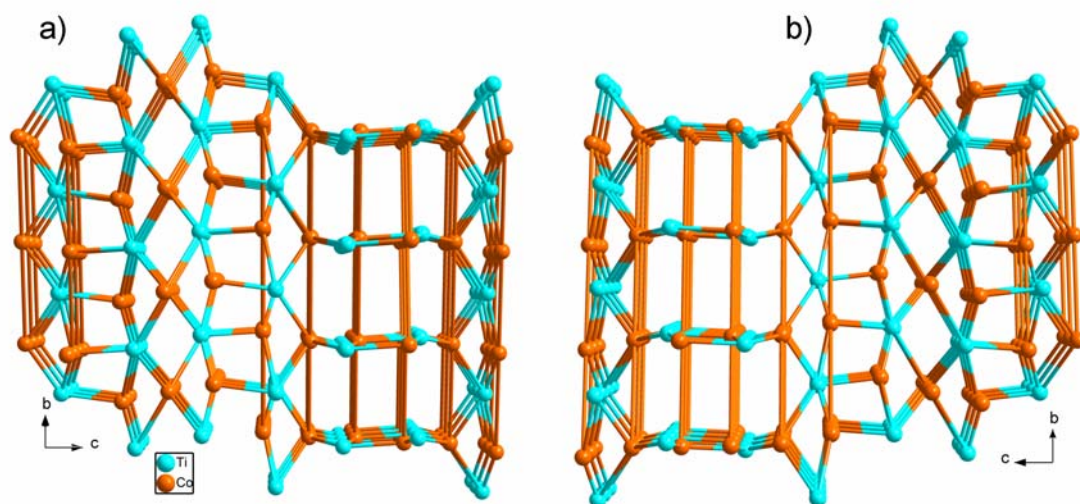
Figure S5. The topological net of 1-D (a) and 1-L (b)
