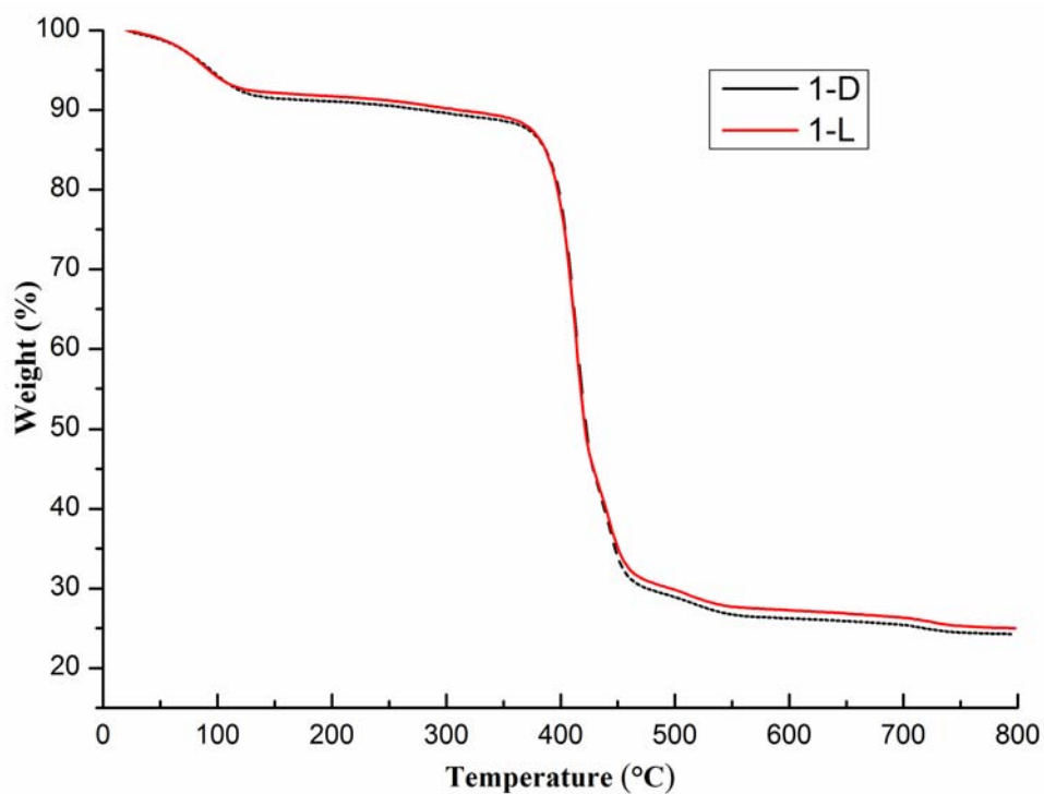
Figure S4. The TGA diagram of 1-D and 1-L
