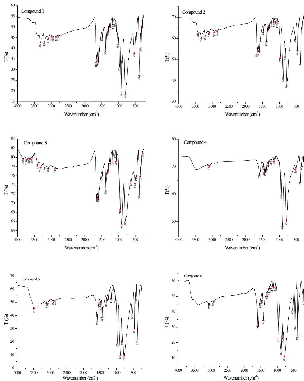
Fig. s1 IR spectra of compounds 1-6.
