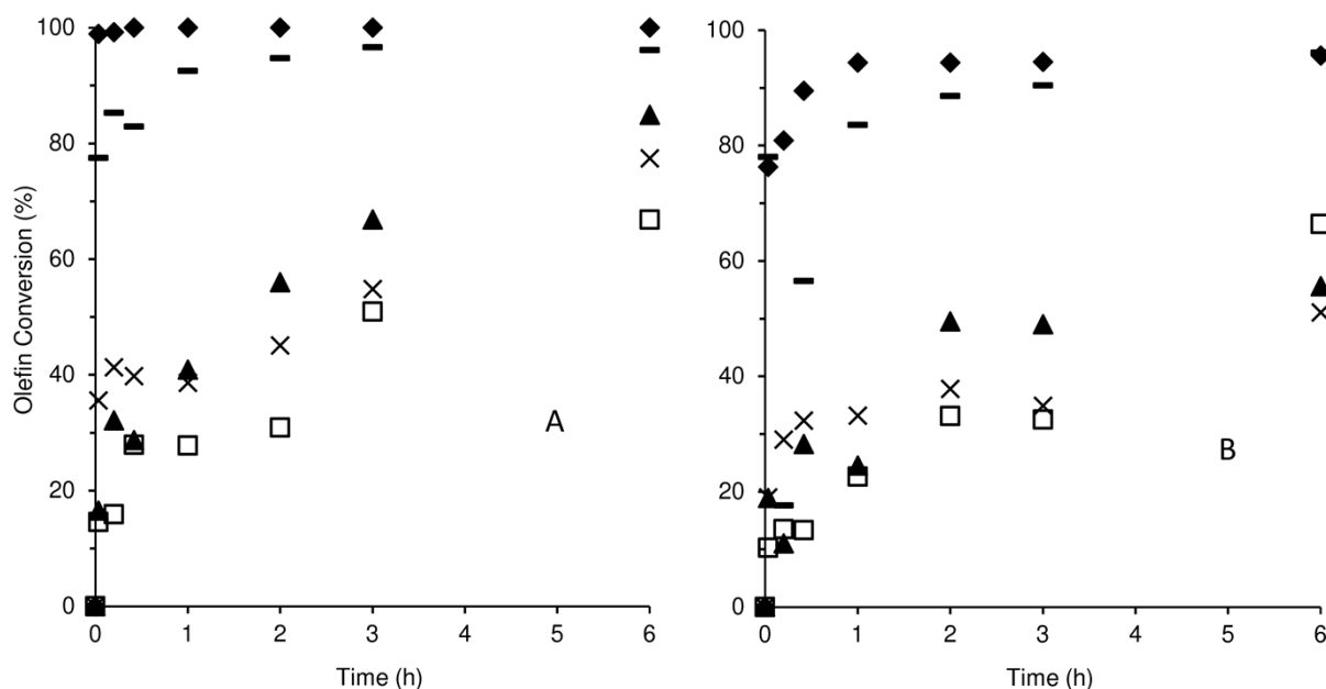
Fig. S1 Oxidation of cis -cyclooctene (◆), 1-octene (□), trans -2-octene (▲), \alpha -pinene (×) and ( R )-(+)-limonene (—) with TBHP using complexes 2 (A) and 3 (B) as catalyst precursors at 55 °C, without cosolvent.
