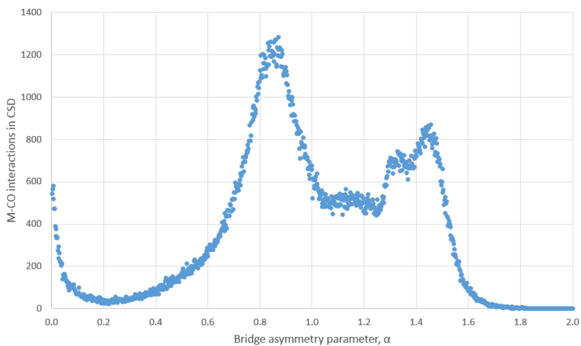
Figure S2. Histogram of CSD entries as a function of the bridging asymmetry parameter, inclusive of all binuclear and polynuclear entries in the CSD.
