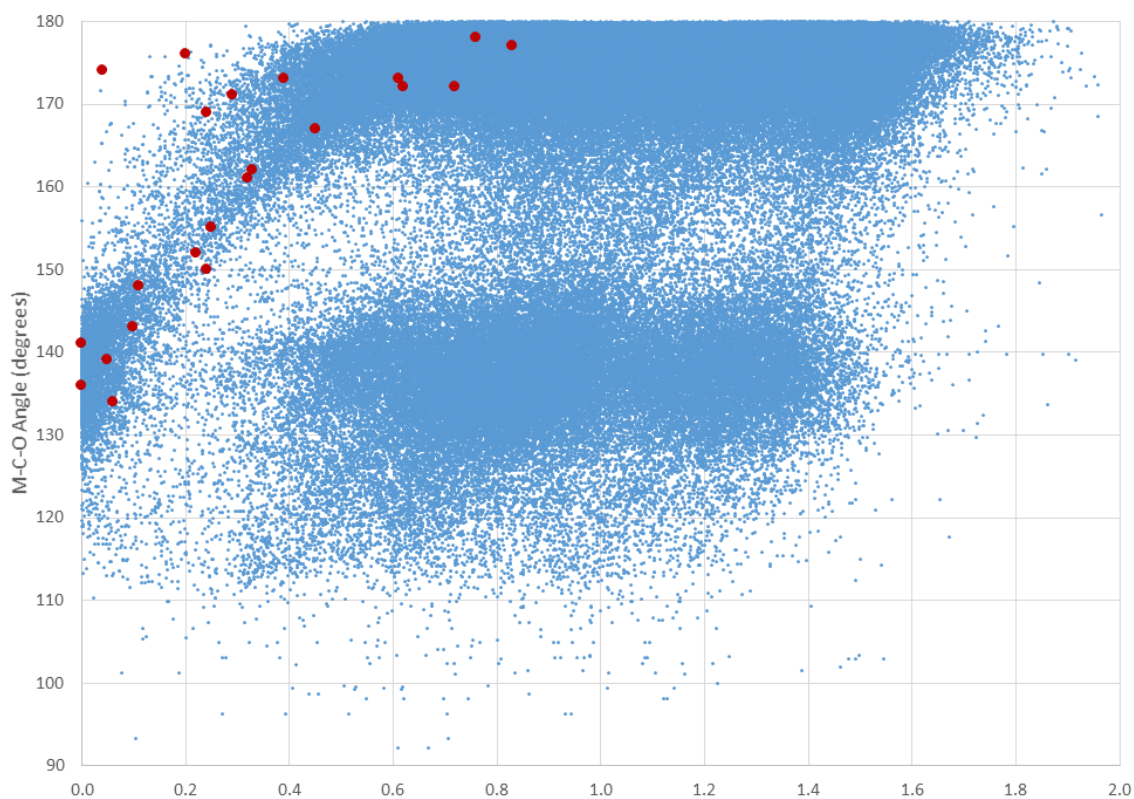
Figure S1. Updated plot of bridging angle as a function of Curtis's bridge asymmetry parameter, inclusive of all binuclear and polynuclear entries in the CSD. Data from the CSD is shown in blue. Curtis's original data points are shown in red.
