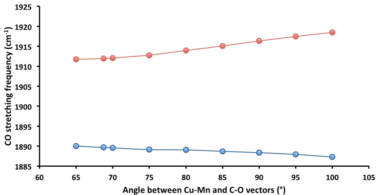
Figure S3. Calculated IR frequencies for (IMe)Cu-Mn(CO) 5 as a function of the angle being varied as shown in Figure 11. Only data for the two vibrational modes involving the SBCO being manipulated are shown.
