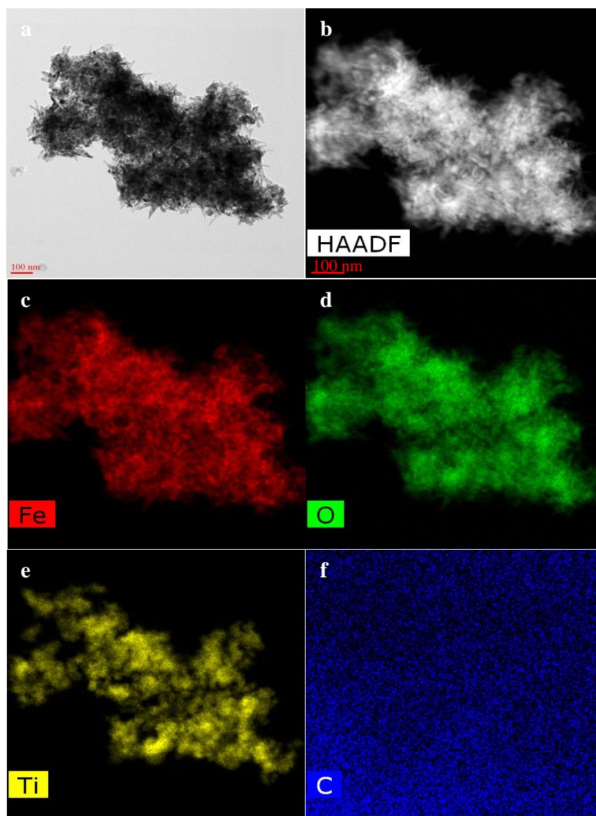
S1 TEM images of (a) ternary composite ( \text{Fe}_2\text{O}_3\text{-TiO}_2/\text{GO}(1.0\ \%) ) from different region, (b) corresponding HAADF STEM image, and the spatially resolved Fe (c), O (d), Ti (e), and C (f) elemental maps of ternary composite
