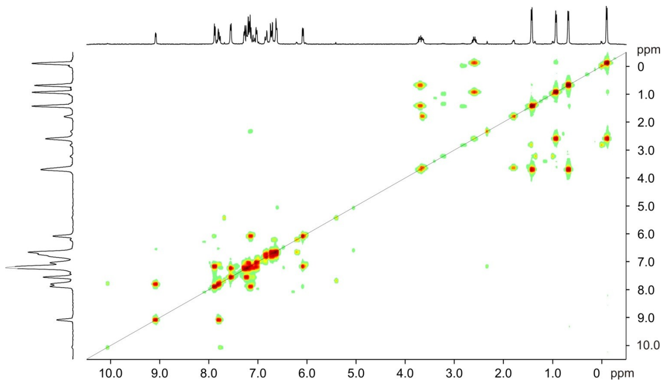
5 Figure S3. ^1\text{H} - ^1\text{H} COSY NMR spectrum of compound 7 in \text{C}_6\text{D}_6 .
