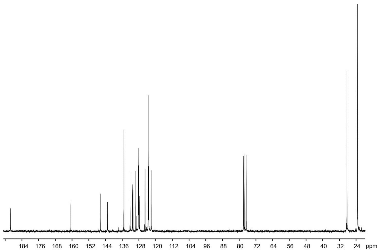
5 Figure S8. ^{13}\text{C} NMR spectrum of compound 3 in \text{CDCl}_3 .
