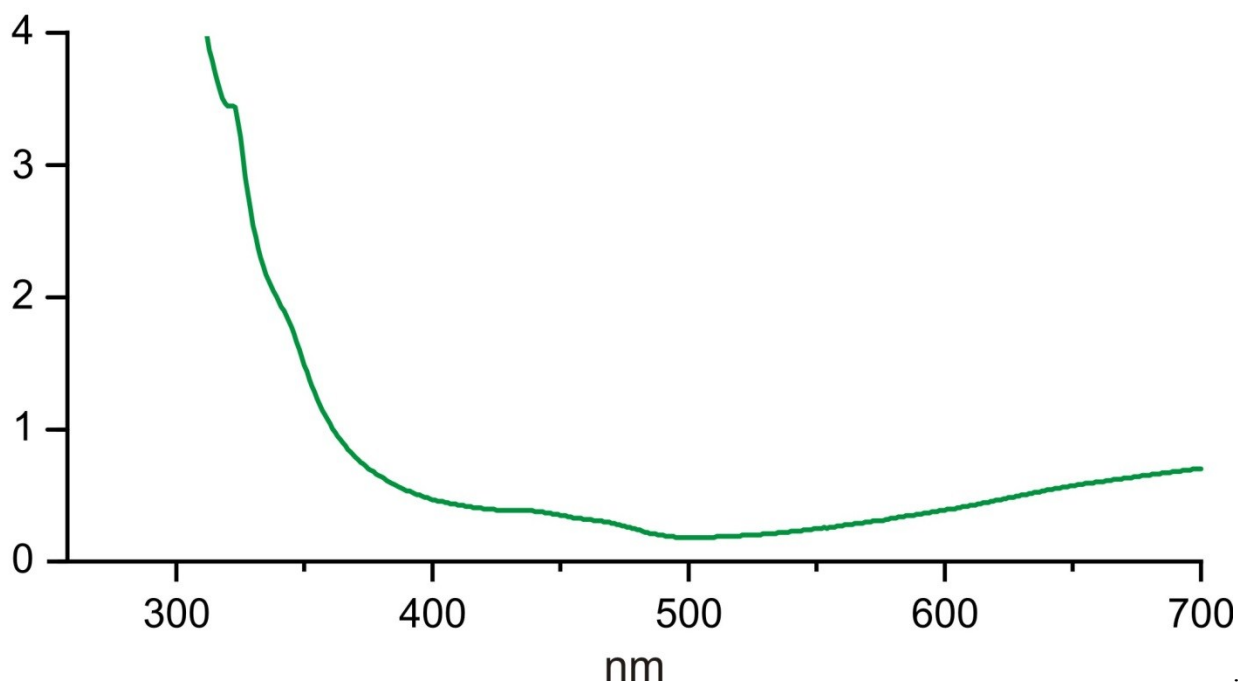
Figure S5. UV-VIS spectrum of compound 4 in THF.
