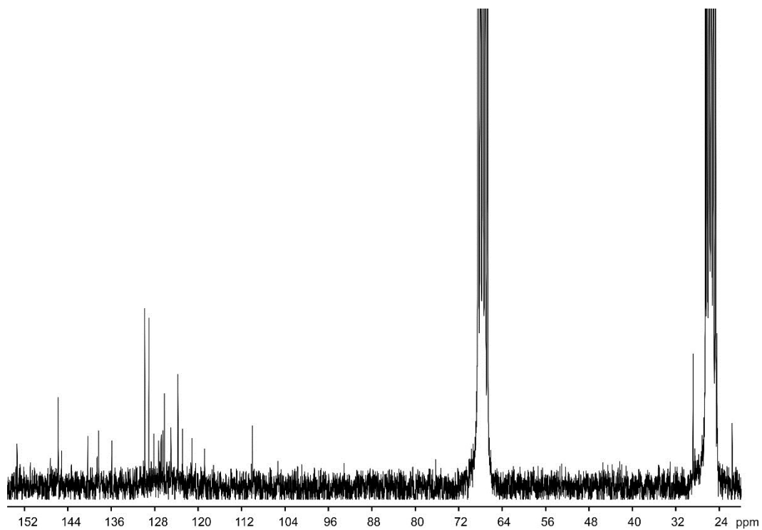
Figure S9. ^{13}\text{C} NMR spectrum of compound 4 in \text{thf-d}_8 .
