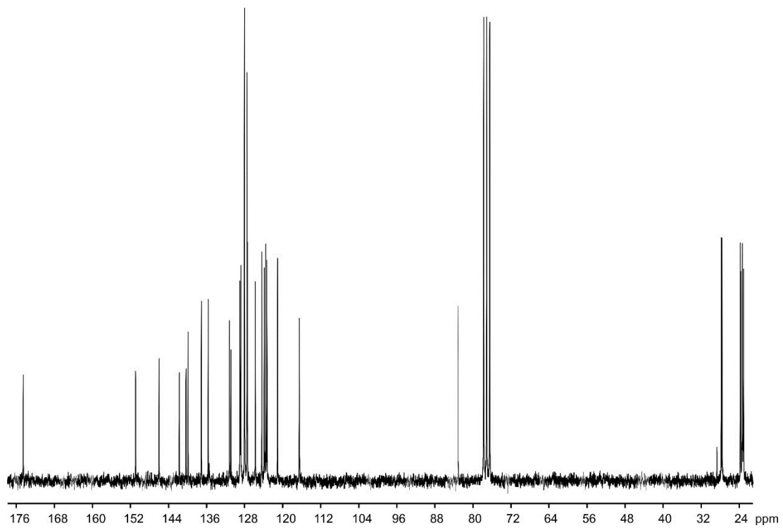
5 Figure S12. ^{13}\text{C} NMR spectrum of compound 8 in \text{CDCl}_3 .
