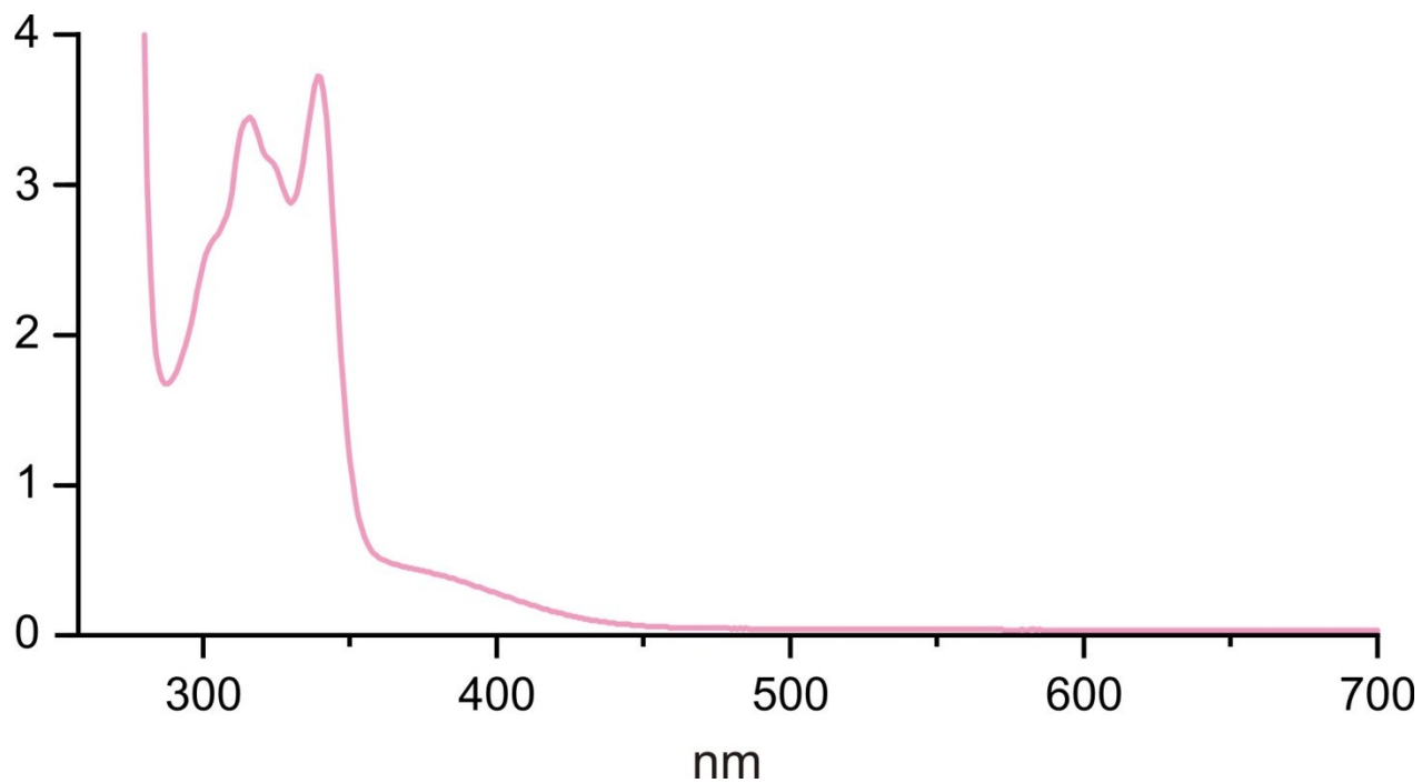
Figure S7. UV-VIS spectrum of compound 7 in toluene.
