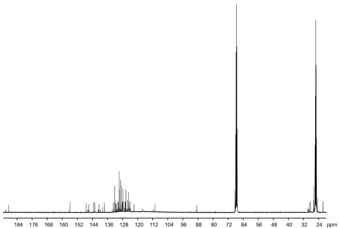
Figure S11. ^{13}\text{C} NMR spectrum of compound 7 in \text{C}_6\text{D}_6 .
