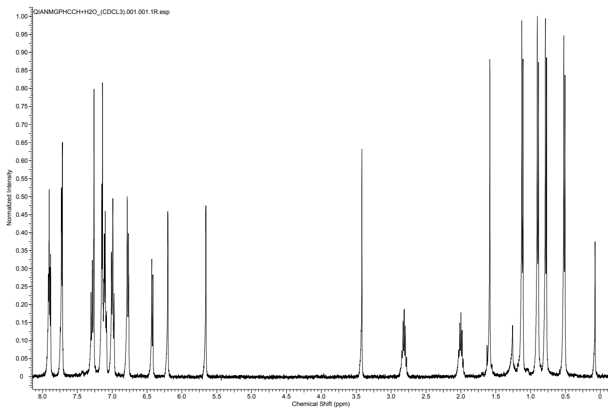
5 Figure S3. ^1\text{H} - ^1\text{H} COSY NMR spectrum of compound 7 in \text{C}_6\text{D}_6 .
