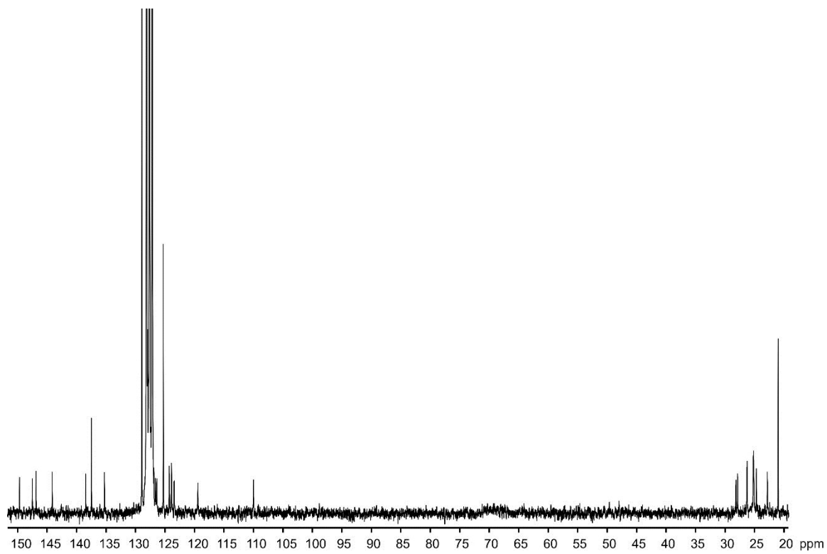
5 Figure S10. ^{13}\text{C} NMR spectrum of compound 5 in \text{C}_6\text{D}_6 .
