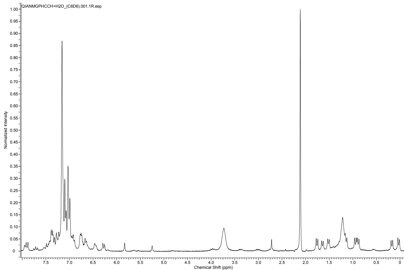
Figure S1. 1 H NMR spectrum of compound 8 in C 6 D 6 .
