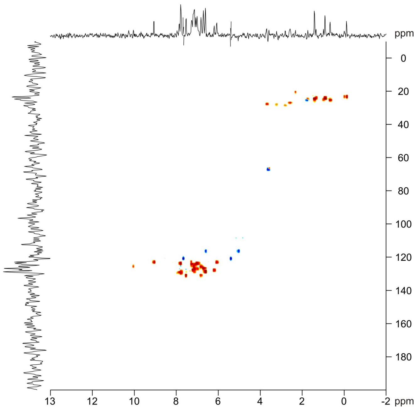
Figure S13. ^1\text{H} - ^{13}\text{C} COSY NMR spectrum of compound 7 in \text{thf-d}_8 .
