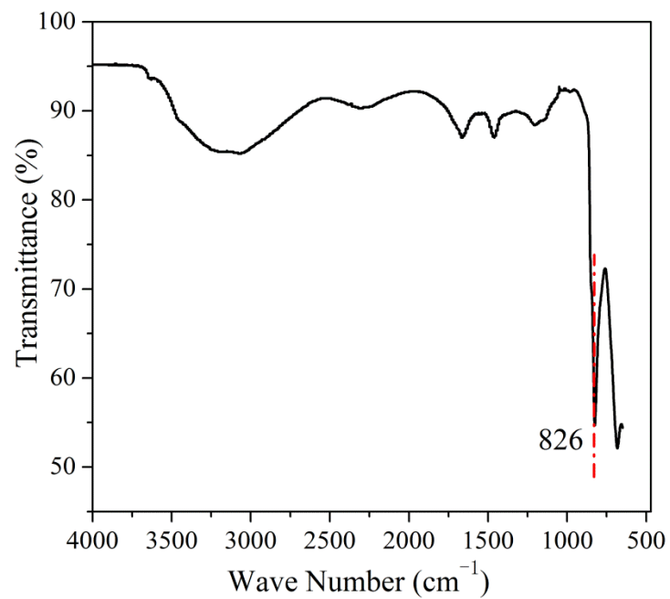
Fig. S1. FTIR spectrum of the dissolved arsenite species in water. Its uncomplexed As(III)-O bond was determined at \sim 826 \text{ cm}^{-1} .
